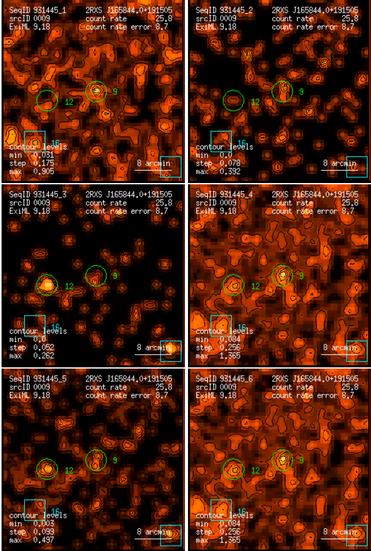
Figure 9: RASS 931445: detection 0009: band rate images, Gaussian filter: (1) PSPC channels 11 – 41, (2) 52 – 90, (3) 91 – 201, (4) 11 – 235, (5) 52 – 201, (6) 11 – 201. Broad band rates in counts/ks. Band rate contour levels in counts/ks/arcmin 2 .
