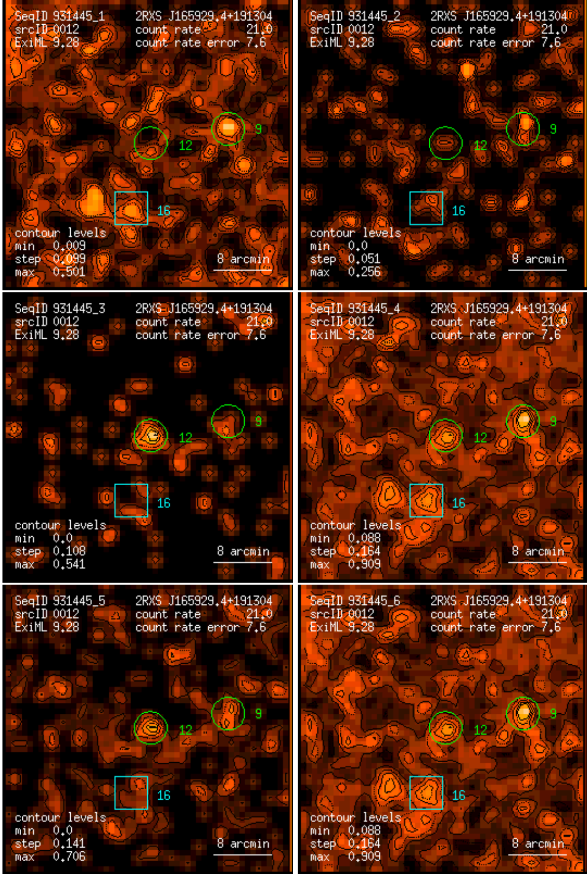
Figure 12: RASS 931445: detection 0012: band rate images, Gaussian filter: (1) PSPC channels 11 – 41, (2) 52 – 90, (3) 91 – 201, (4) 11 – 235, (5) 52 – 201, (6) 11 – 201. Broad band rates in counts/ks. Band rate contour levels in counts/ks/arcmin 2 .
