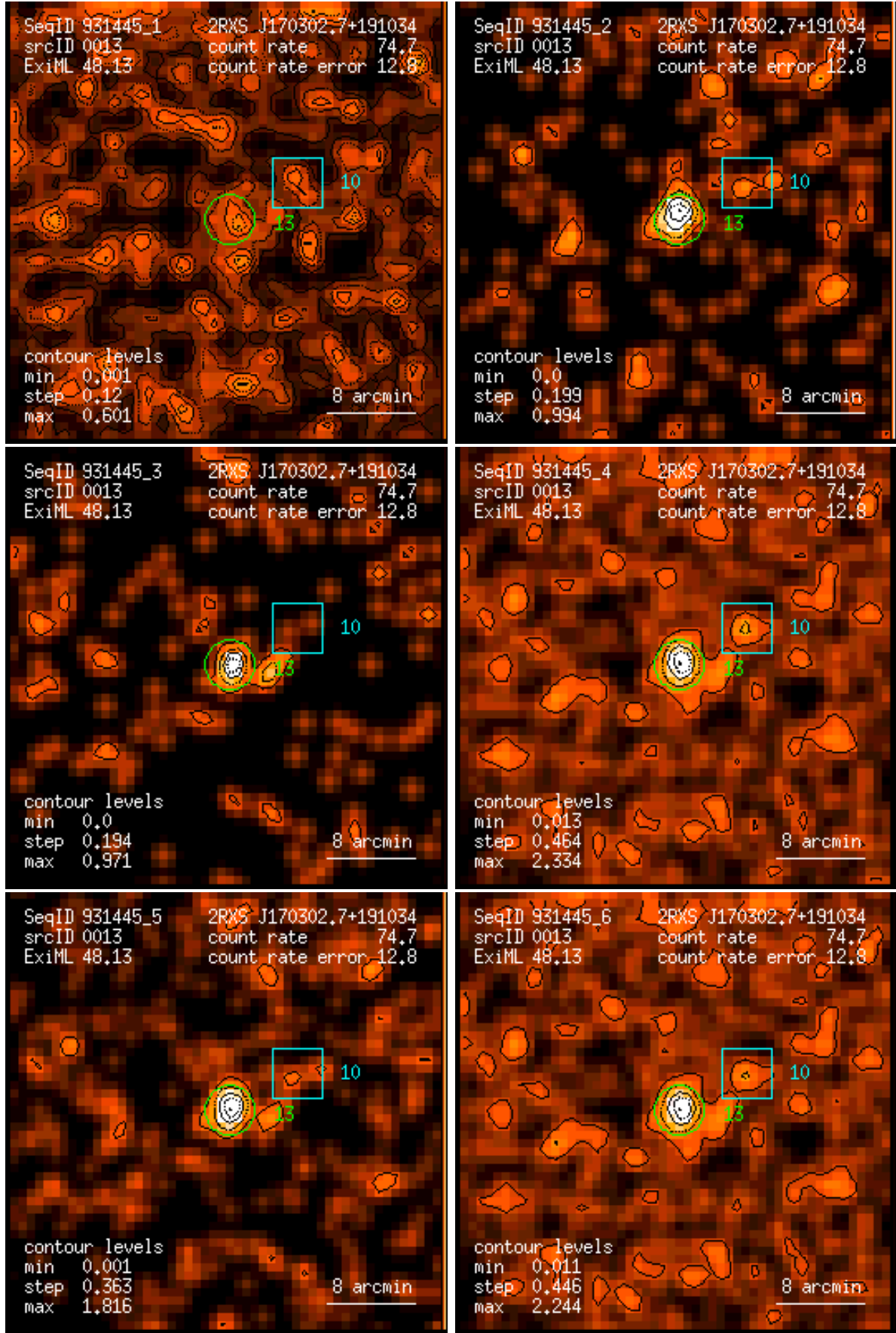
Figure 13: RASS 931445: detection 0013: band rate images, Gaussian filter: (1) PSPC channels 11 – 41, (2) 52 – 90, (3) 91 – 201, (4) 11 – 235, (5) 52 – 201, (6) 11 – 201. Broad band rates in counts/ks. Band rate contour levels in counts/ks/arcmin 2 .
