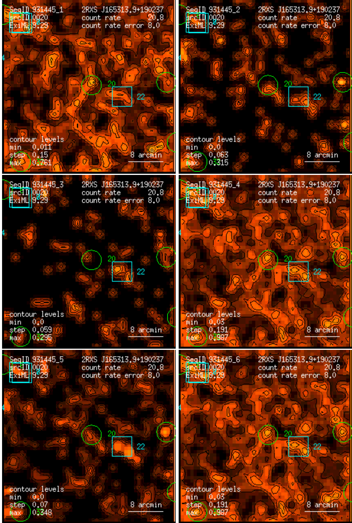
Figure 20: RASS 931445: detection 0020: band rate images, Gaussian filter: (1) PSPC channels 11 – 41, (2) 52 – 90, (3) 91 – 201, (4) 11 – 235, (5) 52 – 201, (6) 11 – 201. Broad band rates in counts/ks. Band rate contour levels in counts/ks/arcmin 2 .
