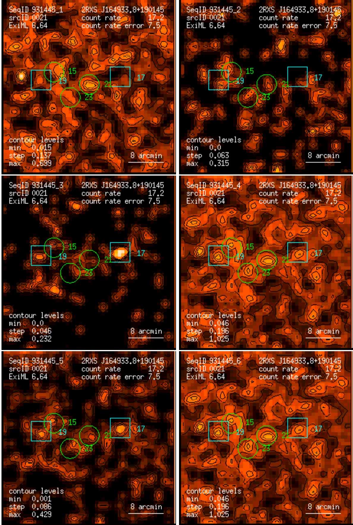
Figure 21: RASS 931445: detection 0021: band rate images, Gaussian filter: (1) PSPC channels 11 – 41, (2) 52 – 90, (3) 91 – 201, (4) 11 – 235, (5) 52 – 201, (6) 11 – 201. Broad band rates in counts/ks. Band rate contour levels in counts/ks/arcmin 2 .
