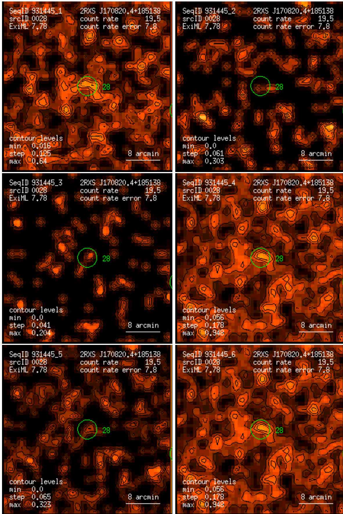
Figure 28: RASS 931445: detection 0028: band rate images, Gaussian filter: (1) PSPC channels 11 – 41, (2) 52 – 90, (3) 91 – 201, (4) 11 – 235, (5) 52 – 201, (6) 11 – 201. Broad band rates in counts/ks. Band rate contour levels in counts/ks/arcmin 2 .
