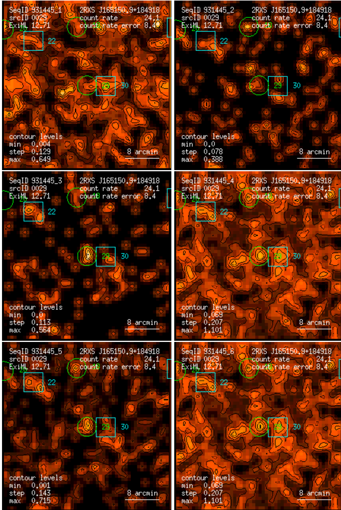
Figure 29: RASS 931445: detection 0029: band rate images, Gaussian filter: (1) PSPC channels 11 – 41, (2) 52 – 90, (3) 91 – 201, (4) 11 – 235, (5) 52 – 201, (6) 11 – 201. Broad band rates in counts/ks. Band rate contour levels in counts/ks/arcmin 2 .
