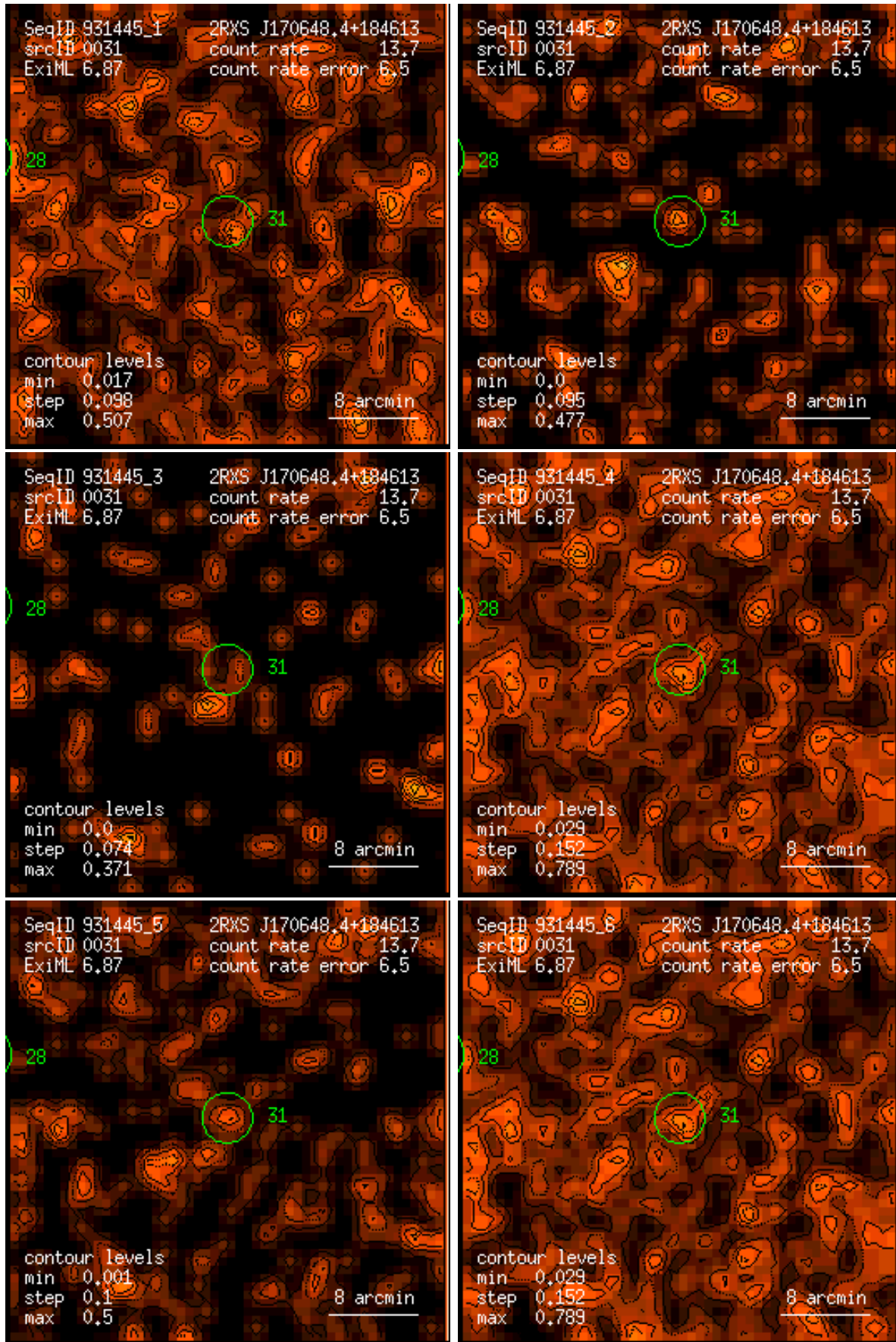
Figure 31: RASS 931445: detection 0031: band rate images, Gaussian filter: (1) PSPP channels 11 – 41, (2) 52 – 90, (3) 91 – 201, (4) 11 – 235, (5) 52 – 201, (6) 11 – 201. Broad band rates in counts/ks. Band rate contour levels in counts/ks/arcmin 2 .
