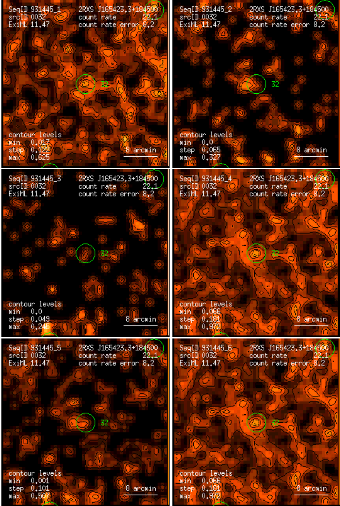
Figure 32: RASS 931445: detection 0032: band rate images, Gaussian filter: (1) PSPC channels 11 – 41, (2) 52 – 90, (3) 91 – 201, (4) 11 – 235, (5) 52 – 201, (6) 11 – 201. Broad band rates in counts/ks. Band rate contour levels in counts/ks/arcmin 2 .
