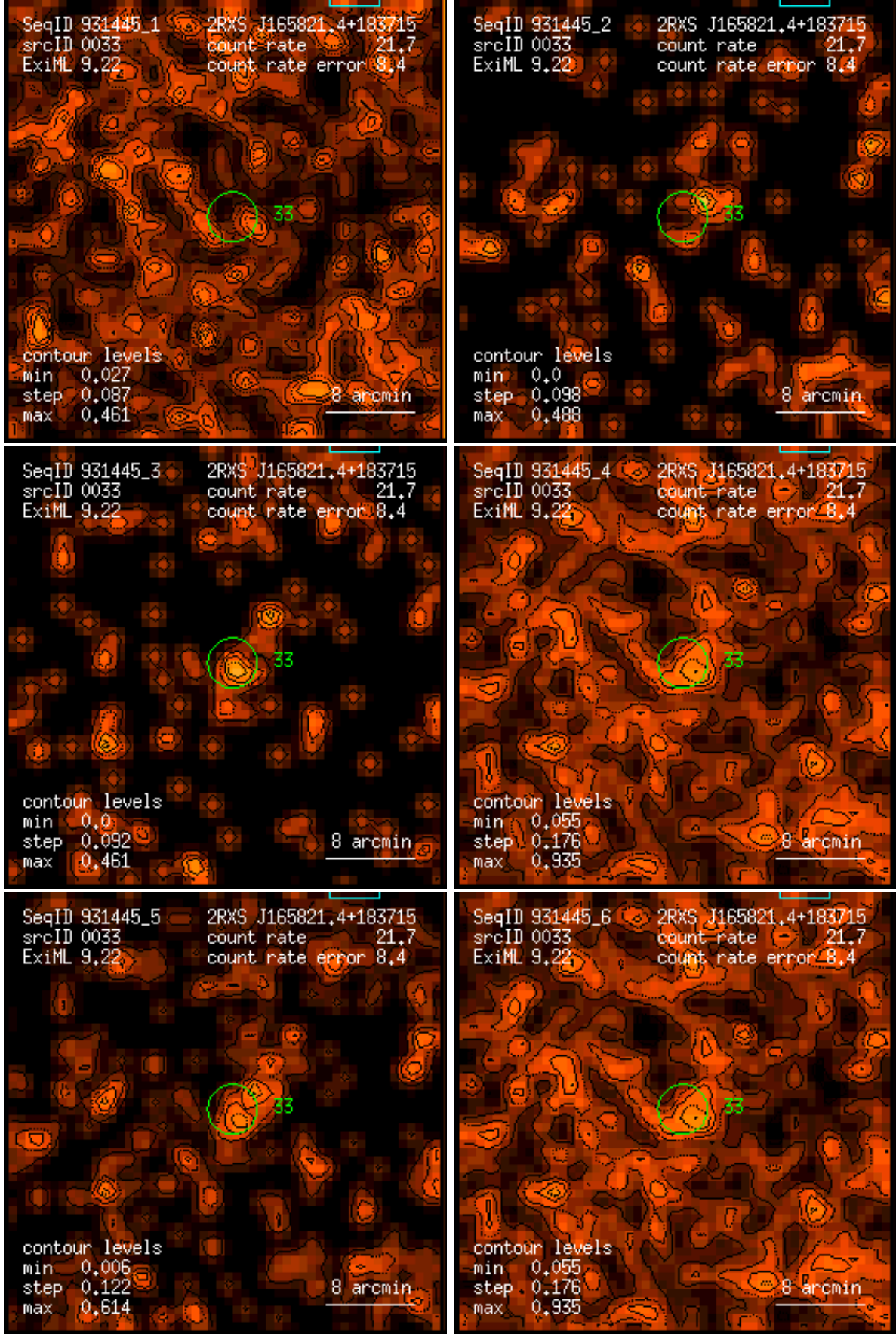
Figure 33: RASS 931445: detection 0033: band rate images, Gaussian filter: (1) PSPC channels 11 – 41, (2) 52 – 90, (3) 91 – 201, (4) 11 – 235, (5) 52 – 201, (6) 11 – 201. Broad band rates in counts/ks. Band rate contour levels in counts/ks/arcmin 2 .
