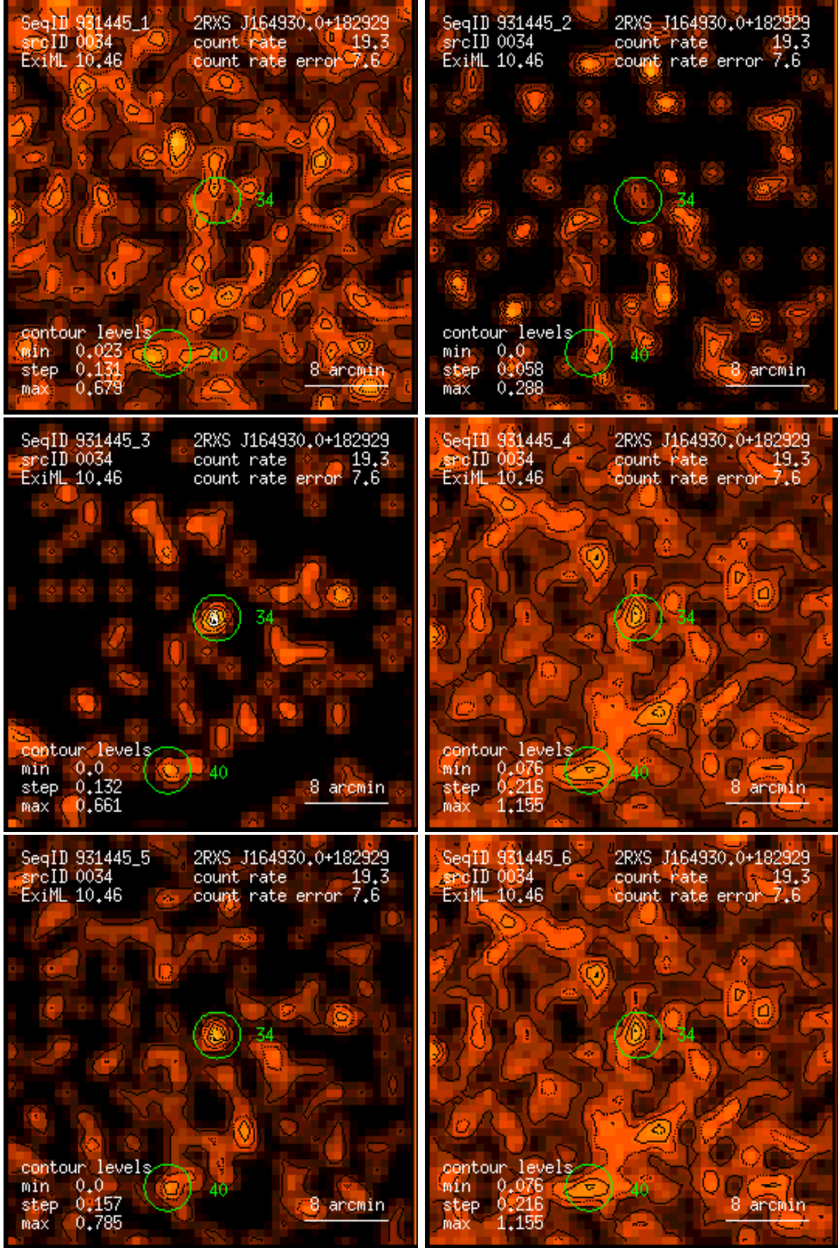
Figure 34: RASS 931445: detection 0034: band rate images, Gaussian filter: (1) PSPC channels 11 – 41, (2) 52 – 90, (3) 91 – 201, (4) 11 – 235, (5) 52 – 201, (6) 11 – 201. Broad band rates in counts/ks. Band rate contour levels in counts/ks/arcmin 2 .
