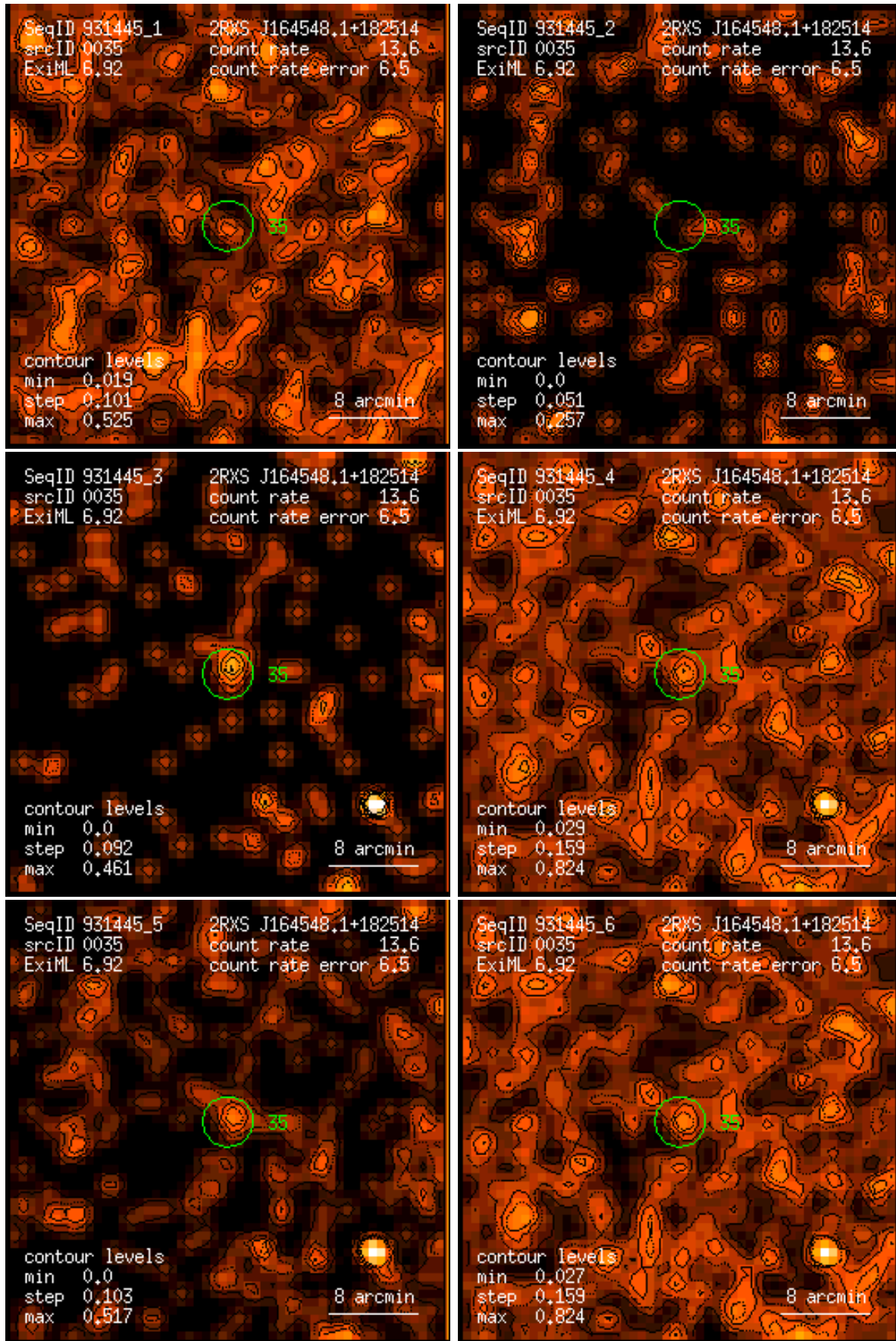
Figure 35: RASS 931445: detection 0035: band rate images, Gaussian filter: (1) PSPC channels 11 – 41, (2) 52 – 90, (3) 91 – 201, (4) 11 – 235, (5) 52 – 201, (6) 11 – 201. Broad band rates in counts/ks. Band rate contour levels in counts/ks/arcmin 2 .
