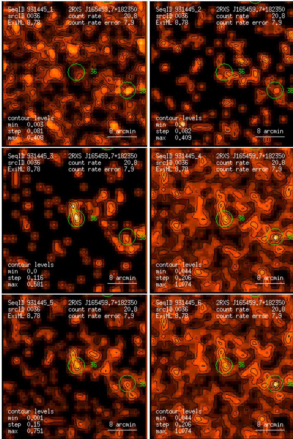
Figure 36: RASS 931445: detection 0036: band rate images, Gaussian filter: (1) PSPC channels 11 – 41, (2) 52 – 90, (3) 91 – 201, (4) 11 – 235, (5) 52 – 201, (6) 11 – 201. Broad band rates in counts/ks. Band rate contour levels in counts/ks/arcmin 2 .
