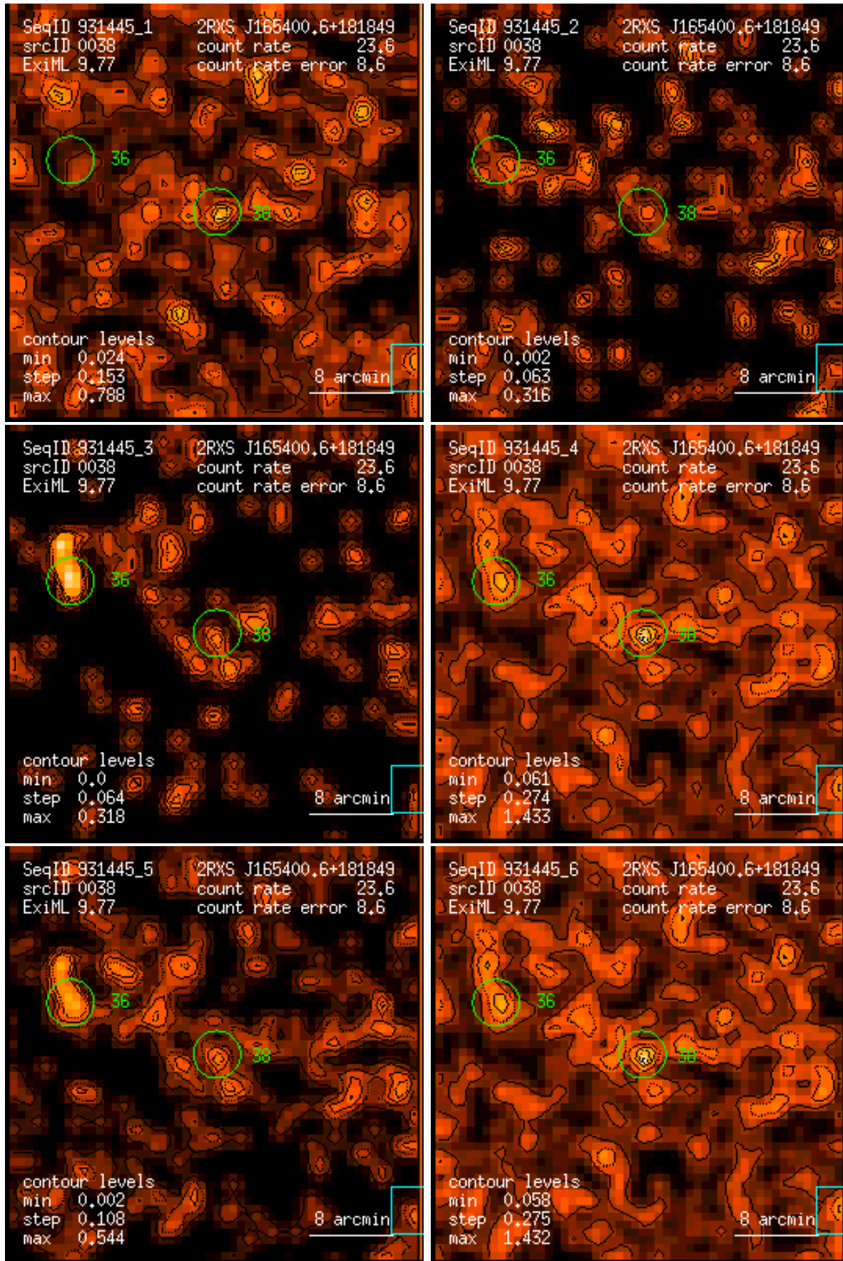
Figure 38: RASS 931445: detection 0038: band rate images, Gaussian filter: (1) PSPC channels 11 – 41, (2) 52 – 90, (3) 91 – 201, (4) 11 – 235, (5) 52 – 201, (6) 11 – 201. Broad band rates in counts/ks. Band rate contour levels in counts/ks/arcmin 2 .
