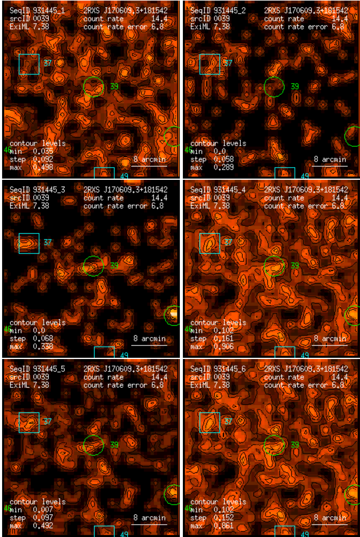
Figure 39: RASS 931445: detection 0039: band rate images, Gaussian filter: (1) PSPC channels 11 – 41, (2) 52 – 90, (3) 91 – 201, (4) 11 – 235, (5) 52 – 201, (6) 11 – 201. Broad band rates in counts/ks. Band rate contour levels in counts/ks/arcmin 2 .
