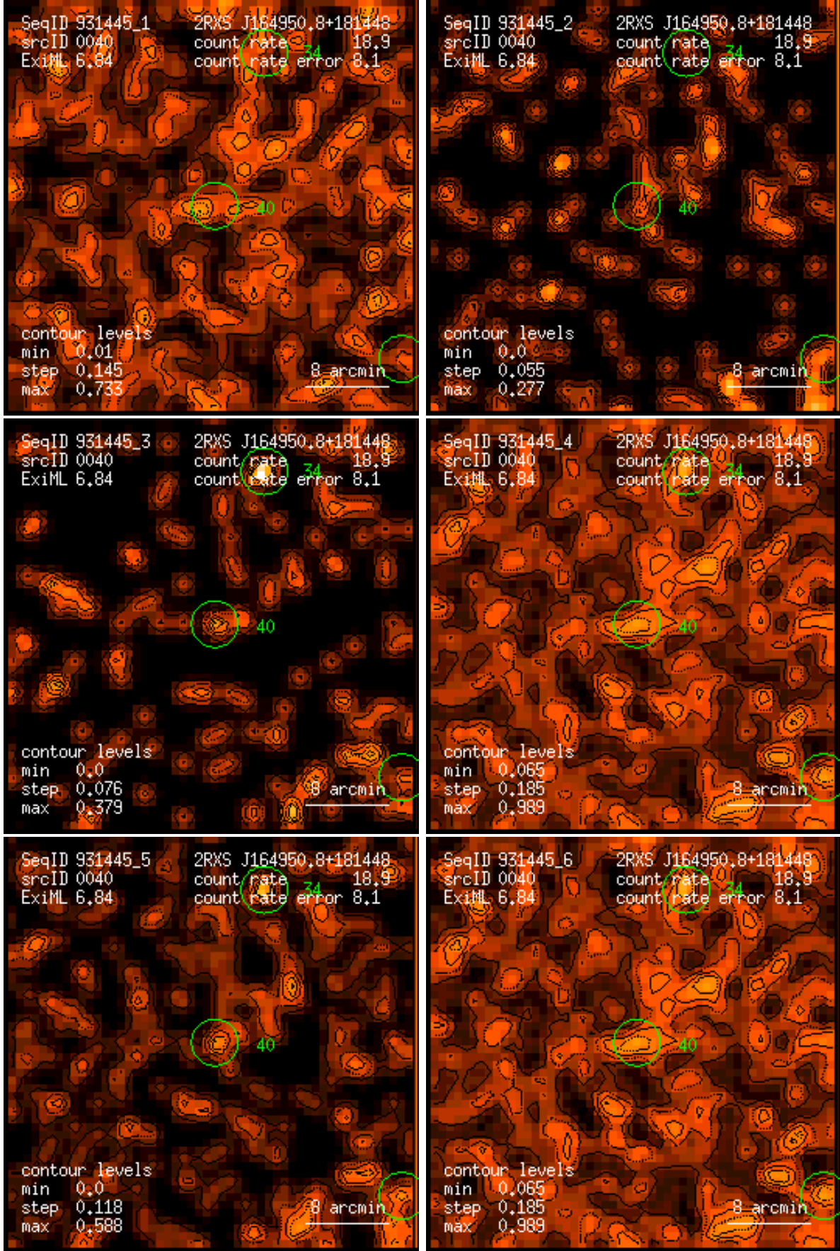
Figure 40: RASS 931445: detection 0040: band rate images, Gaussian filter: (1) PSPC channels 11 – 41, (2) 52 – 90, (3) 91 – 201, (4) 11 – 235, (5) 52 – 201, (6) 11 – 201. Broad band rates in counts/ks. Band rate contour levels in counts/ks/arcmin 2 .
