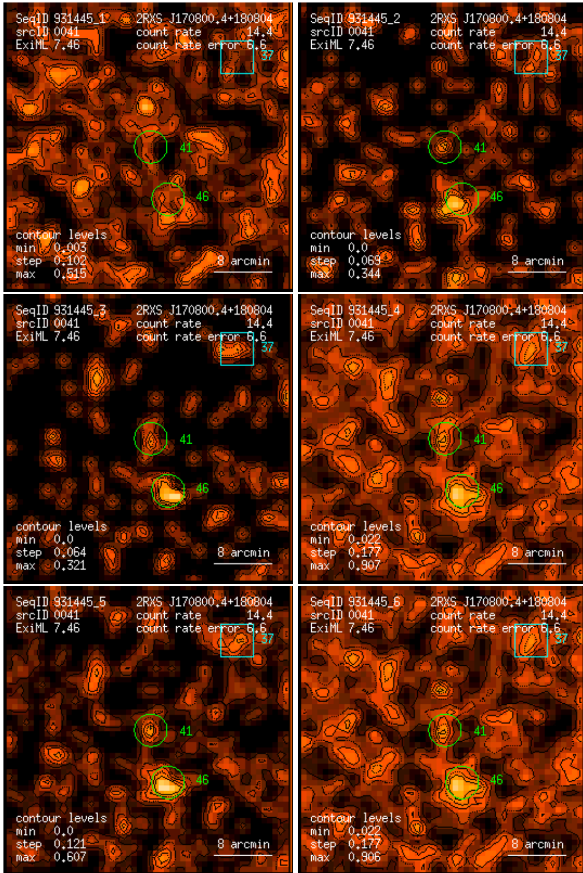
Figure 41: RASS 931445: detection 0041: band rate images, Gaussian filter: (1) PSPC channels 11 – 41, (2) 52 – 90, (3) 91 – 201, (4) 11 – 235, (5) 52 – 201, (6) 11 – 201. Broad band rates in counts/ks. Band rate contour levels in counts/ks/arcmin 2 .
