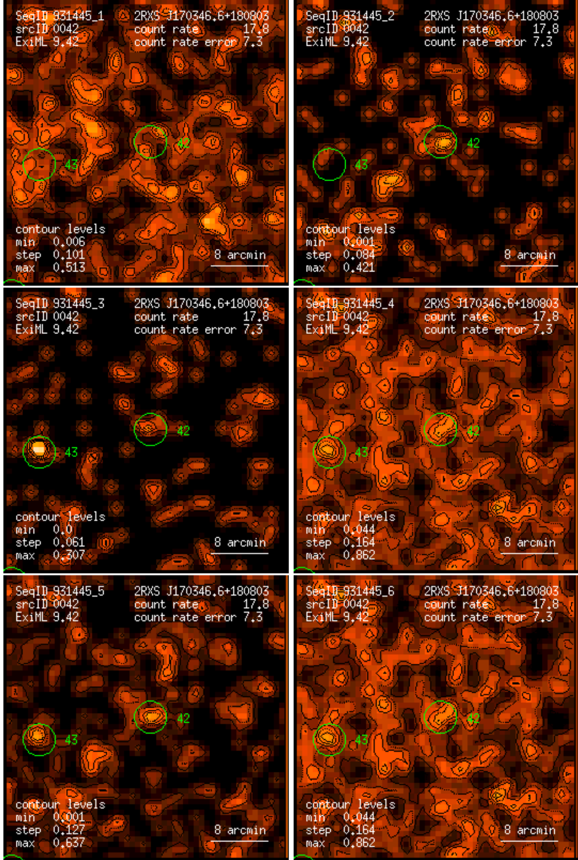
Figure 42: RASS 931445: detection 0042: band rate images, Gaussian filter: (1) PSPC channels 11 – 41, (2) 52 – 90, (3) 91 – 201, (4) 11 – 235, (5) 52 – 201, (6) 11 – 201. Broad band rates in counts/ks. Band rate contour levels in counts/ks/arcmin 2 .
