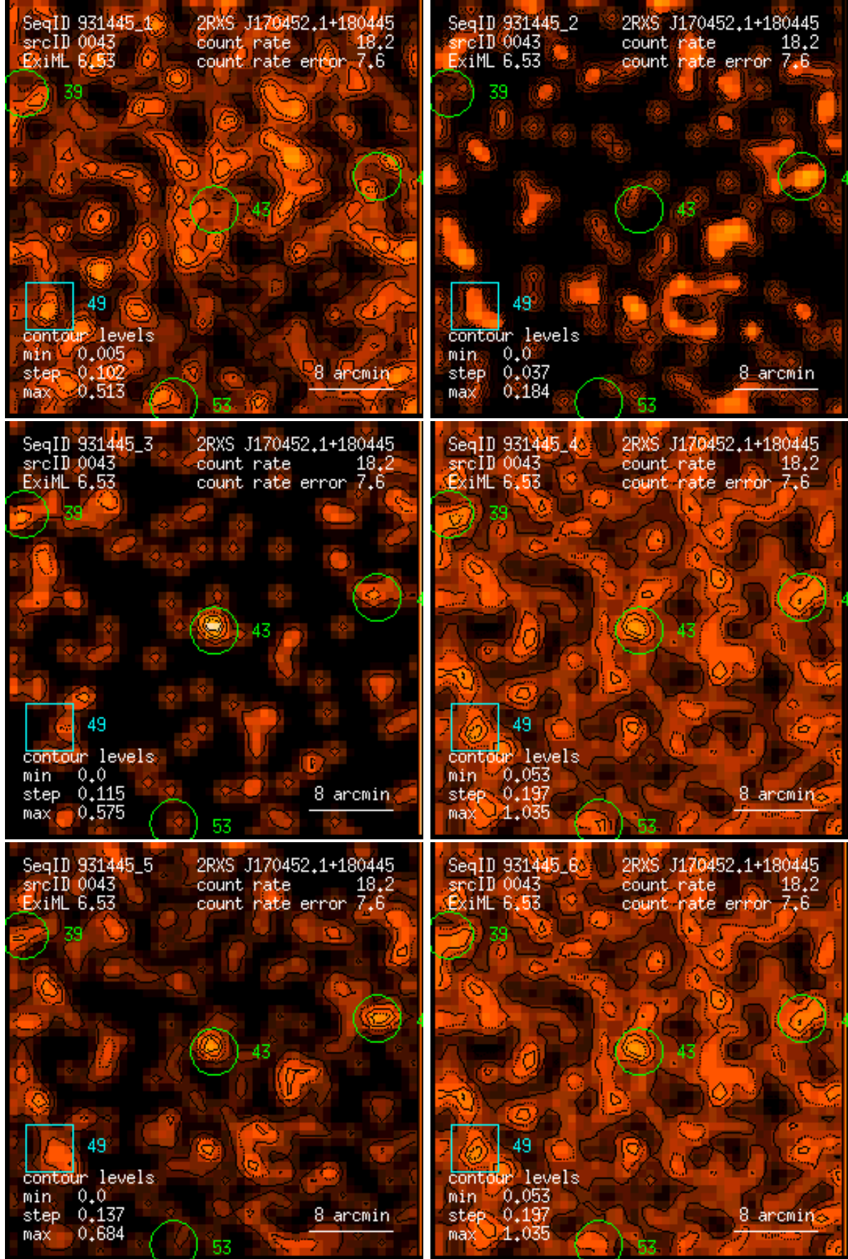
Figure 43: RASS 931445: detection 0043: band rate images, Gaussian filter: (1) PSPC channels 11 – 41, (2) 52 – 90, (3) 91 – 201, (4) 11 – 235, (5) 52 – 201, (6) 11 – 201. Broad band rates in counts/ks. Band rate contour levels in counts/ks/arcmin 2 .
