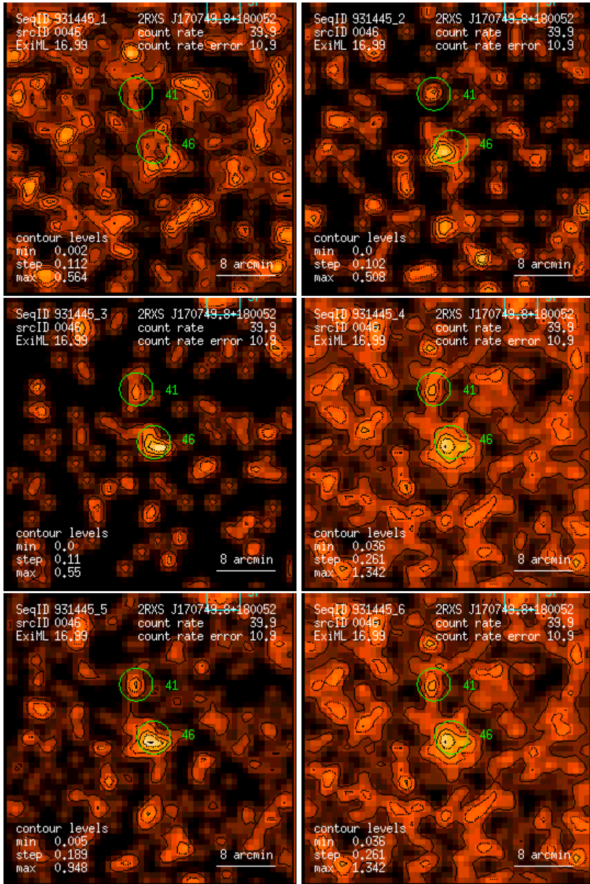
Figure 46: RASS 931445: detection 0046: band rate images, Gaussian filter: (1) PSPC channels 11 – 41, (2) 52 – 90, (3) 91 – 201, (4) 11 – 235, (5) 52 – 201, (6) 11 – 201. Broad band rates in counts/ks. Band rate contour levels in counts/ks/arcmin 2 .
