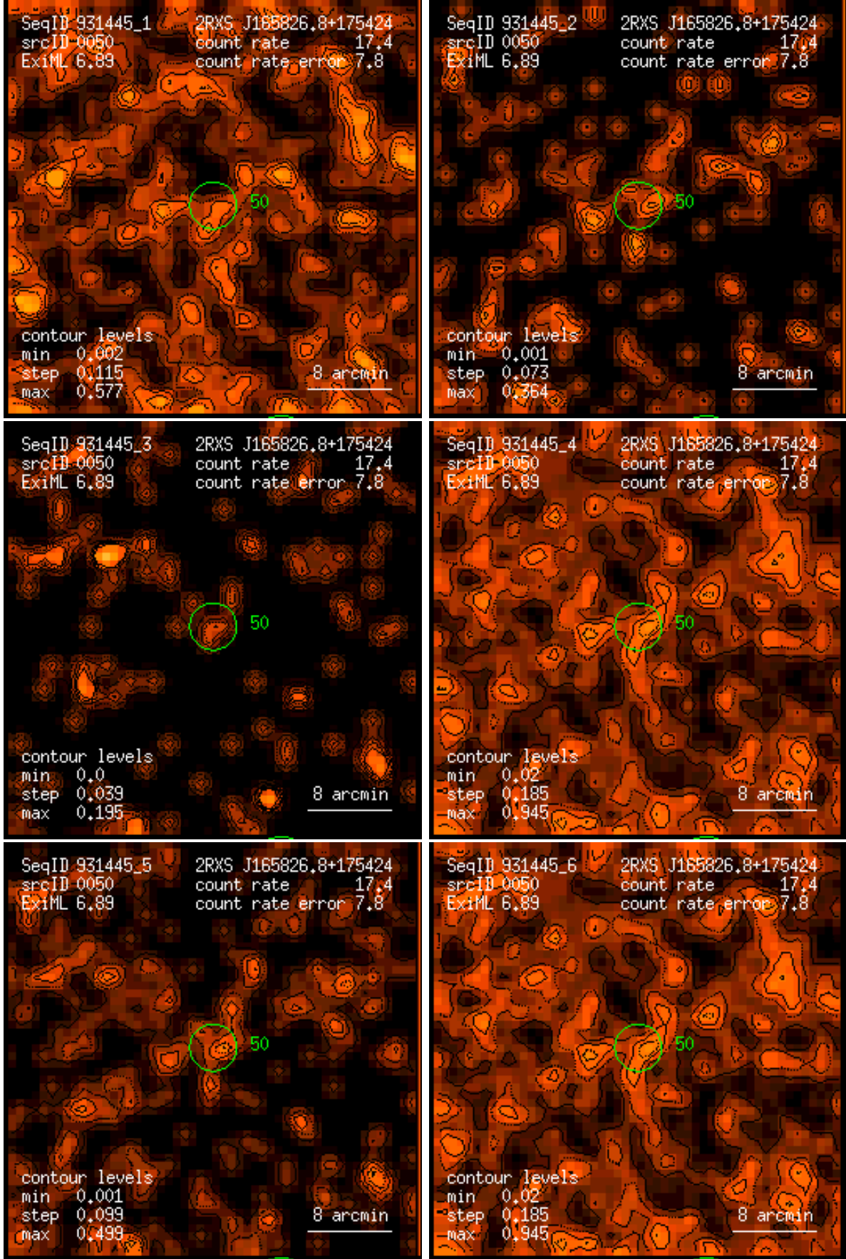
Figure 50: RASS 931445: detection 0050: band rate images, Gaussian filter: (1) PSPC channels 11 – 41, (2) 52 – 90, (3) 91 – 201, (4) 11 – 235, (5) 52 – 201, (6) 11 – 201. Broad band rates in counts/ks. Band rate contour levels in counts/ks/arcmin 2 .
