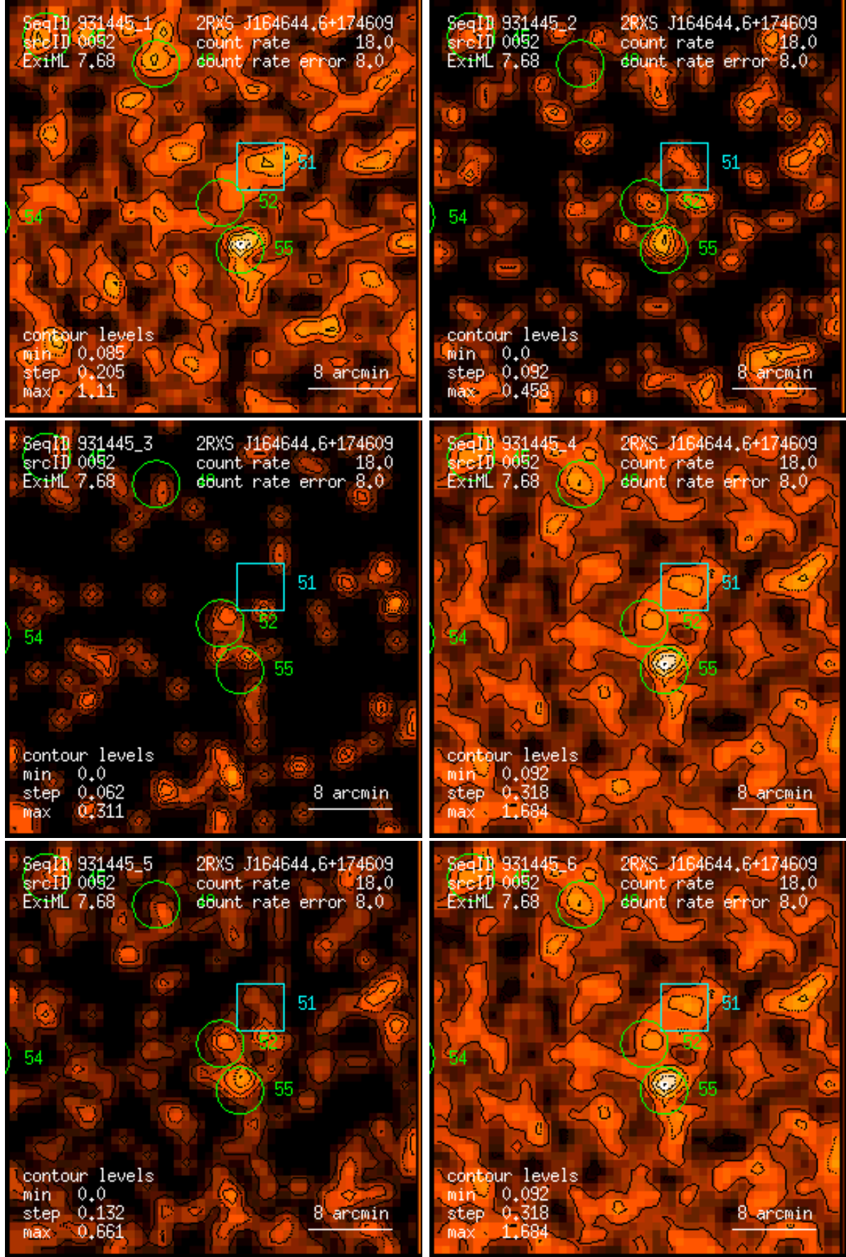
Figure 52: RASS 931445: detection 0052: band rate images, Gaussian filter: (1) PSPC channels 11 – 41, (2) 52 – 90, (3) 91 – 201, (4) 11 – 235, (5) 52 – 201, (6) 11 – 201. Broad band rates in counts/ks. Band rate contour levels in counts/ks/arcmin 2 .
