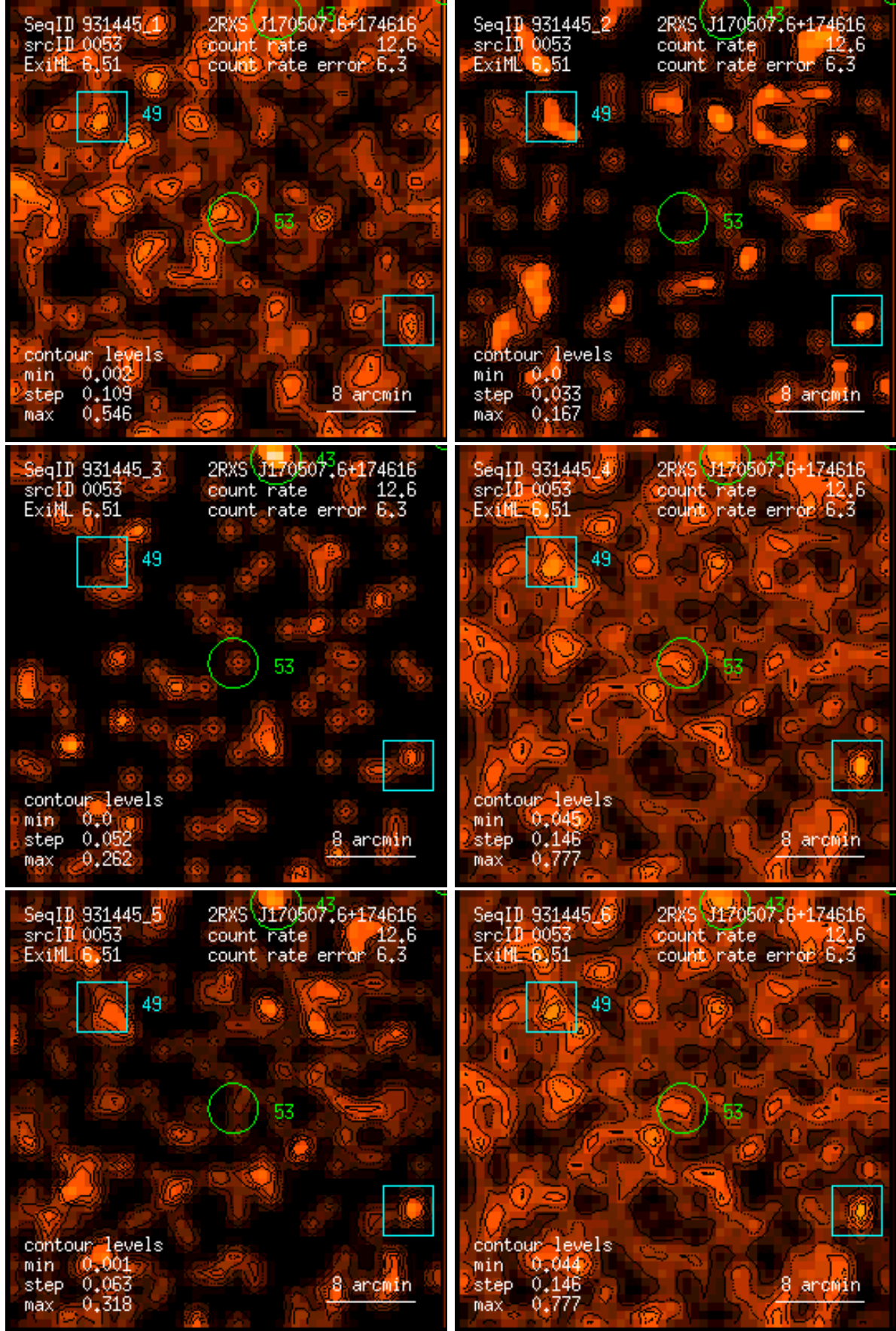
Figure 53: RASS 931445: detection 0053: band rate images, Gaussian filter: (1) PSPC channels 11 – 41, (2) 52 – 90, (3) 91 – 201, (4) 11 – 235, (5) 52 – 201, (6) 11 – 201. Broad band rates in counts/ks. Band rate contour levels in counts/ks/arcmin 2 .
