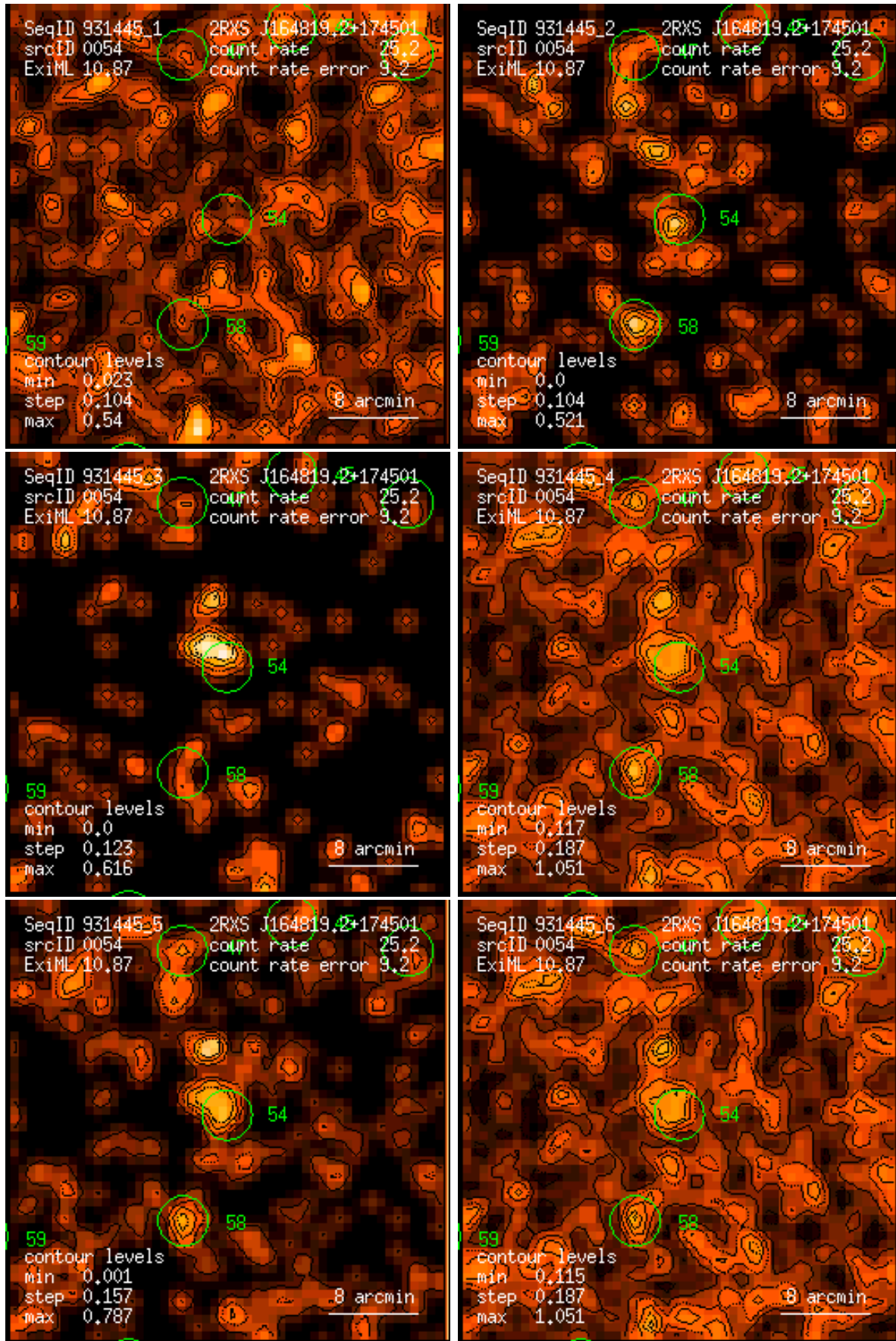
Figure 54: RASS 931445: detection 0054: band rate images, Gaussian filter: (1) PSPC channels 11 – 41, (2) 52 – 90, (3) 91 – 201, (4) 11 – 235, (5) 52 – 201, (6) 11 – 201. Broad band rates in counts/ks. Band rate contour levels in counts/ks/arcmin 2 .
