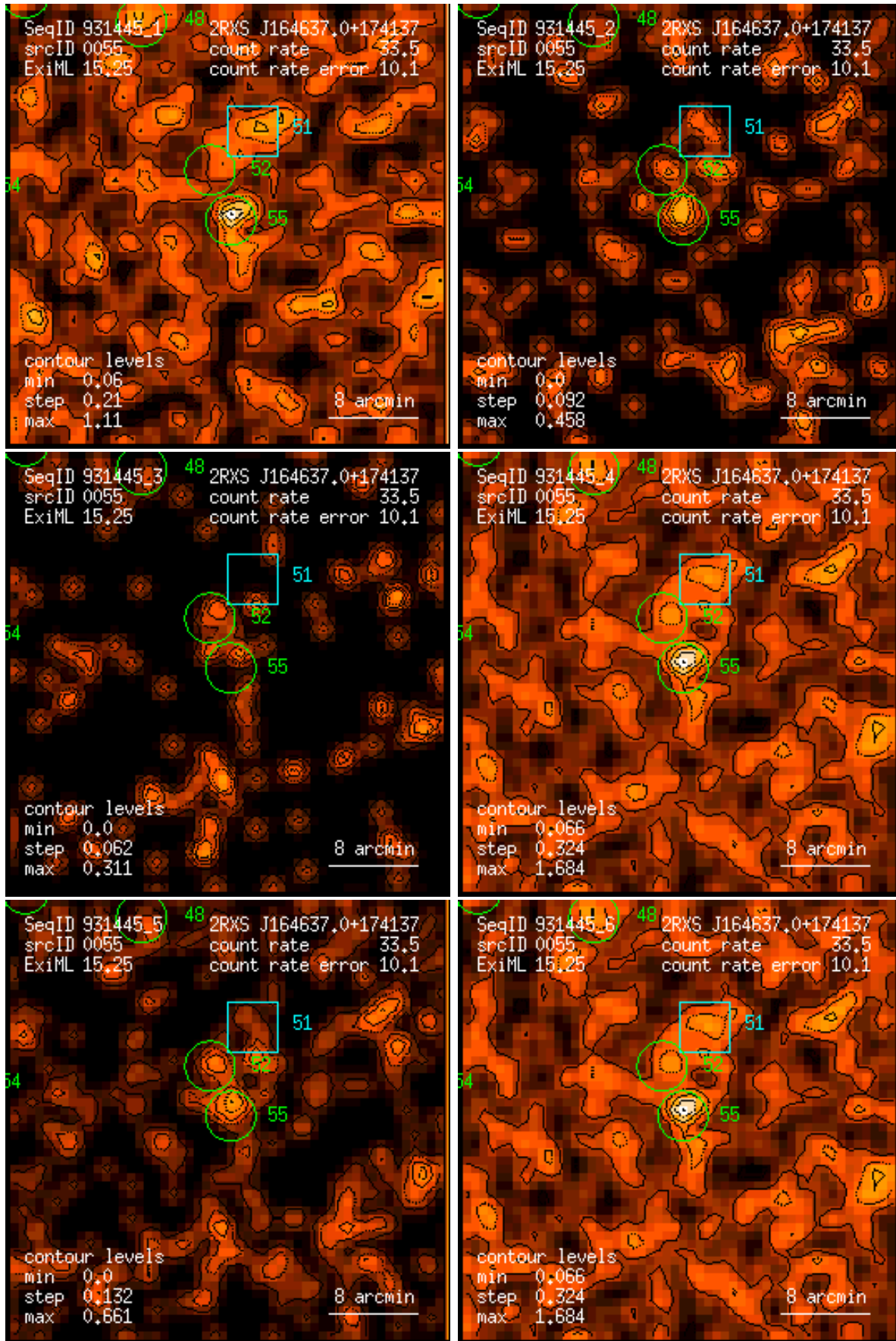
Figure 55: RASS 931445: detection 0055: band rate images, Gaussian filter: (1) PSPC channels 11 – 41, (2) 52 – 90, (3) 91 – 201, (4) 11 – 235, (5) 52 – 201, (6) 11 – 201. Broad band rates in counts/ks. Band rate contour levels in counts/ks/arcmin 2 .
