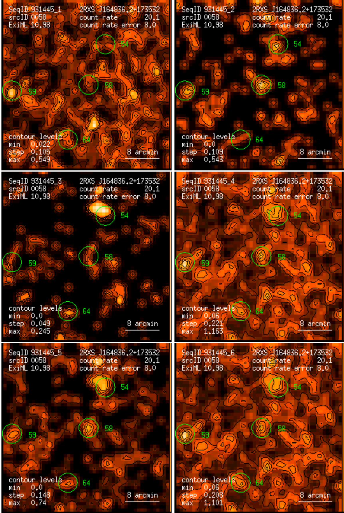
Figure 58: RASS 931445: detection 0058: band rate images, Gaussian filter: (1) PSPC channels 11 – 41, (2) 52 – 90, (3) 91 – 201, (4) 11 – 235, (5) 52 – 201, (6) 11 – 201. Broad band rates in counts/ks. Band rate contour levels in counts/ks/arcmin 2 .
