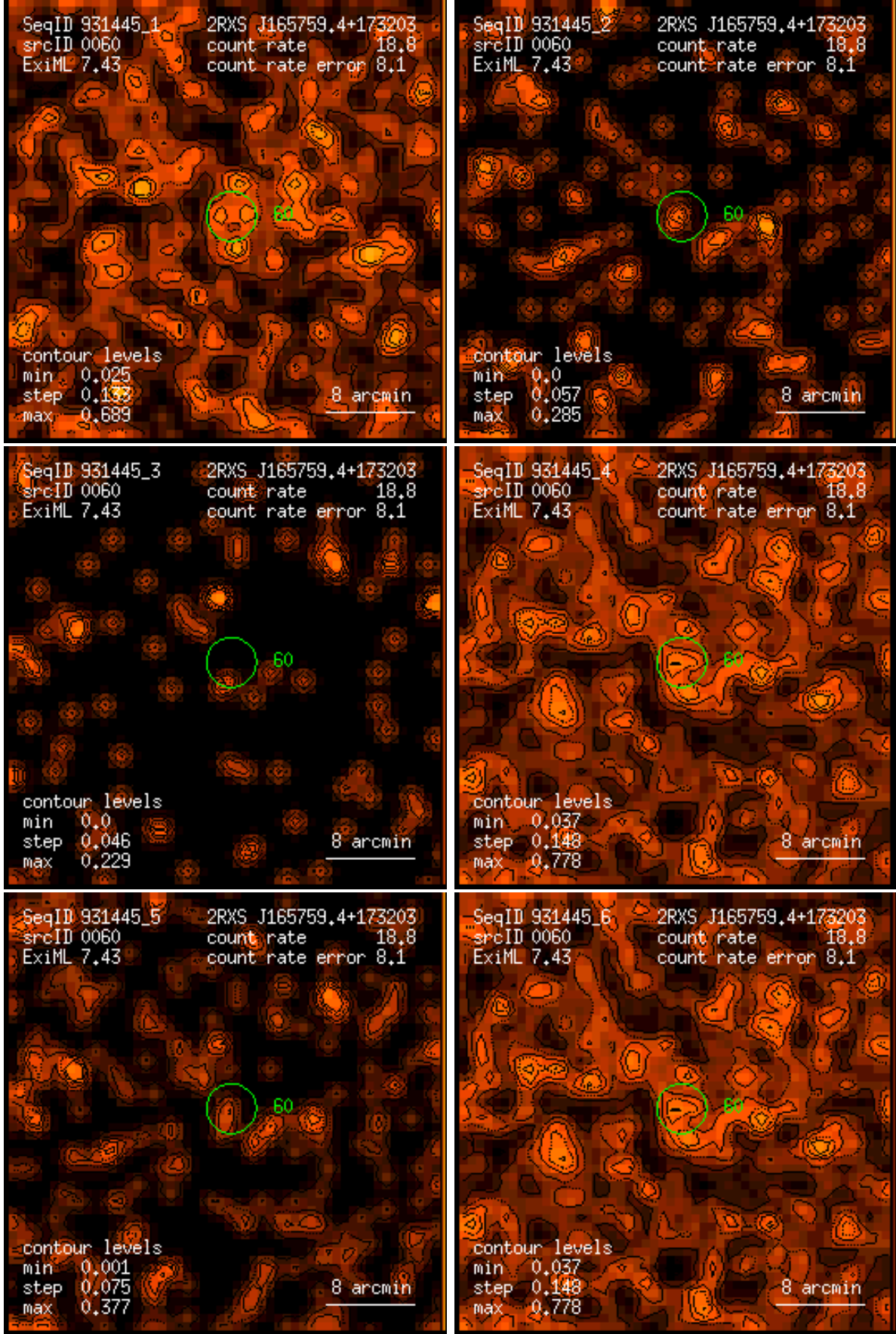
Figure 60: RASS 931445: detection 0060: band rate images, Gaussian filter: (1) PSPC channels 11 – 41, (2) 52 – 90, (3) 91 – 201, (4) 11 – 235, (5) 52 – 201, (6) 11 – 201. Broad band rates in counts/ks. Band rate contour levels in counts/ks/arcmin 2 .
