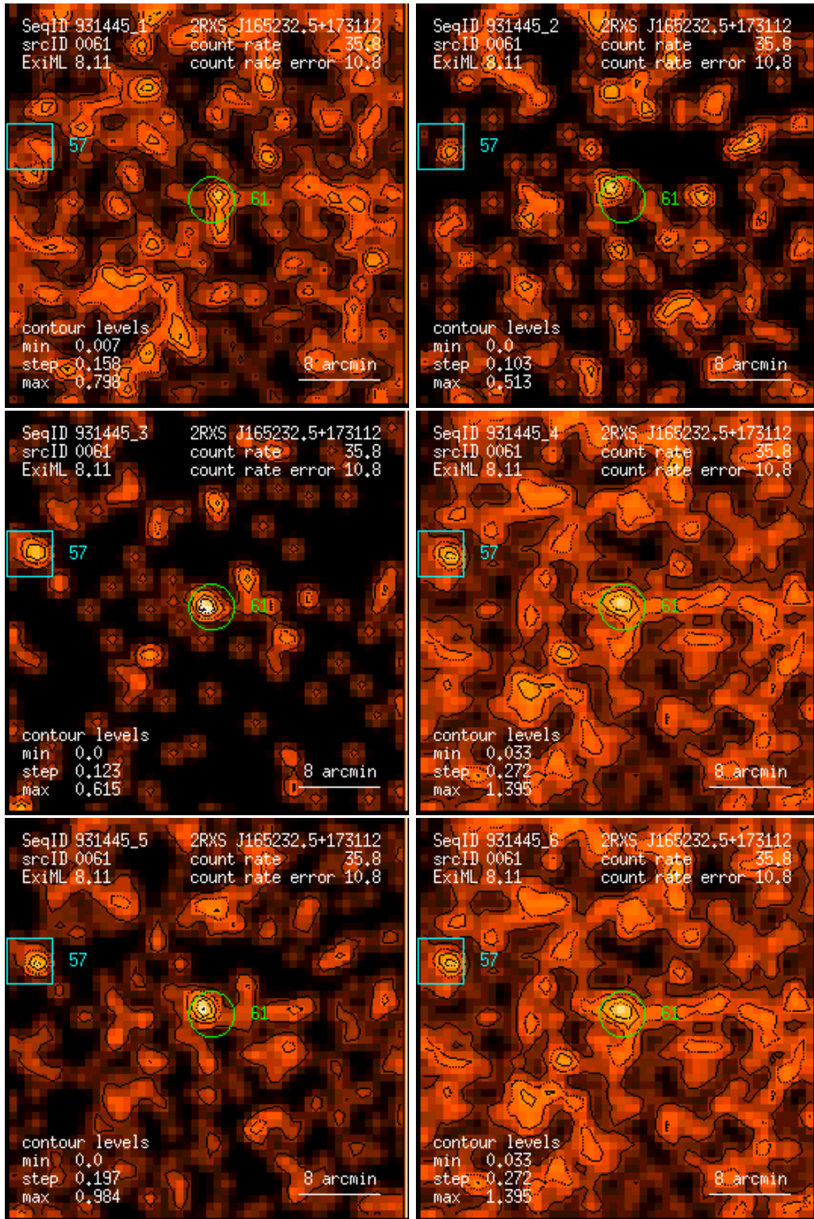
Figure 61: RASS 931445: detection 0061: band rate images, Gaussian filter: (1) PSPC channels 11 – 41, (2) 52 – 90, (3) 91 – 201, (4) 11 – 235, (5) 52 – 201, (6) 11 – 201. Broad band rates in counts/ks. Band rate contour levels in counts/ks/arcmin 2 .
