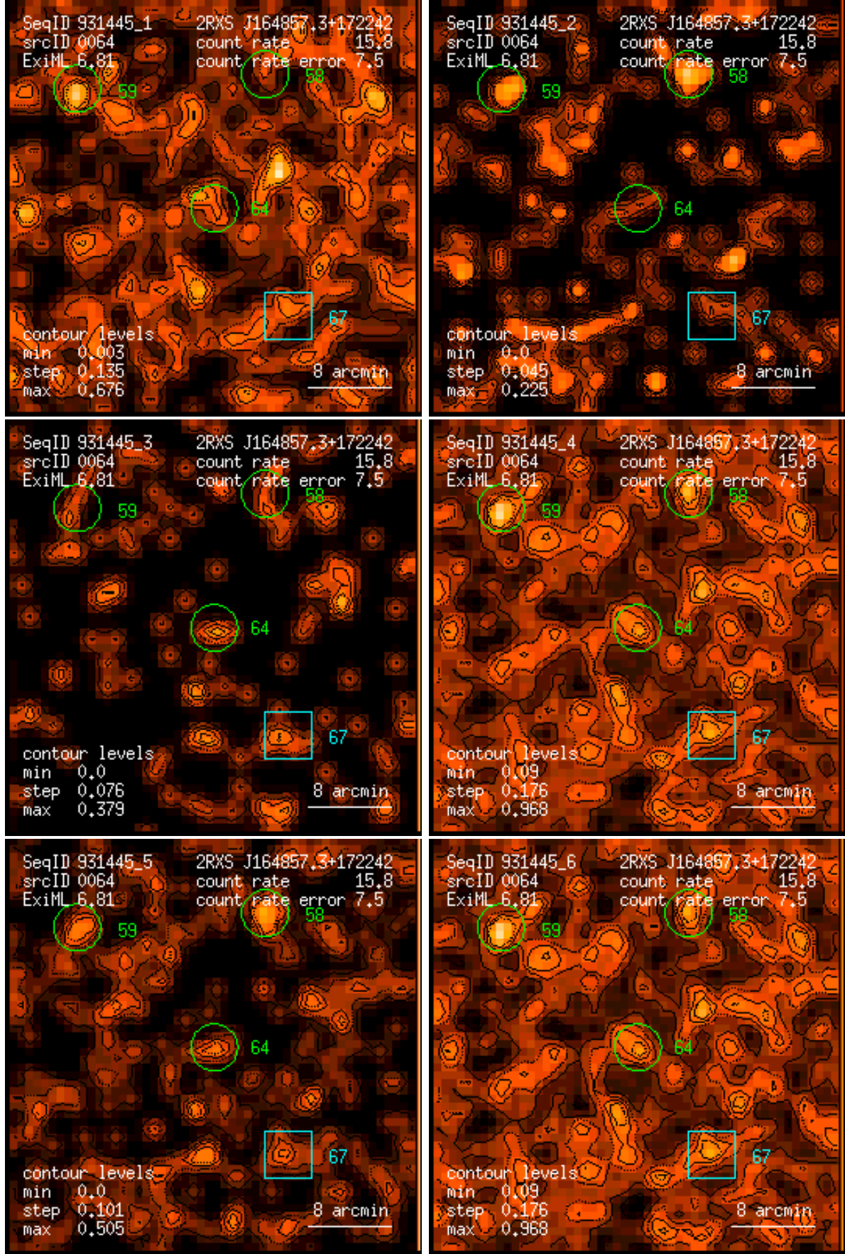
Figure 64: RASS 931445: detection 0064: band rate images, Gaussian filter: (1) PSPC channels 11 – 41, (2) 52 – 90, (3) 91 – 201, (4) 11 – 235, (5) 52 – 201, (6) 11 – 201. Broad band rates in counts/ks. Band rate contour levels in counts/ks/arcmin 2 .
