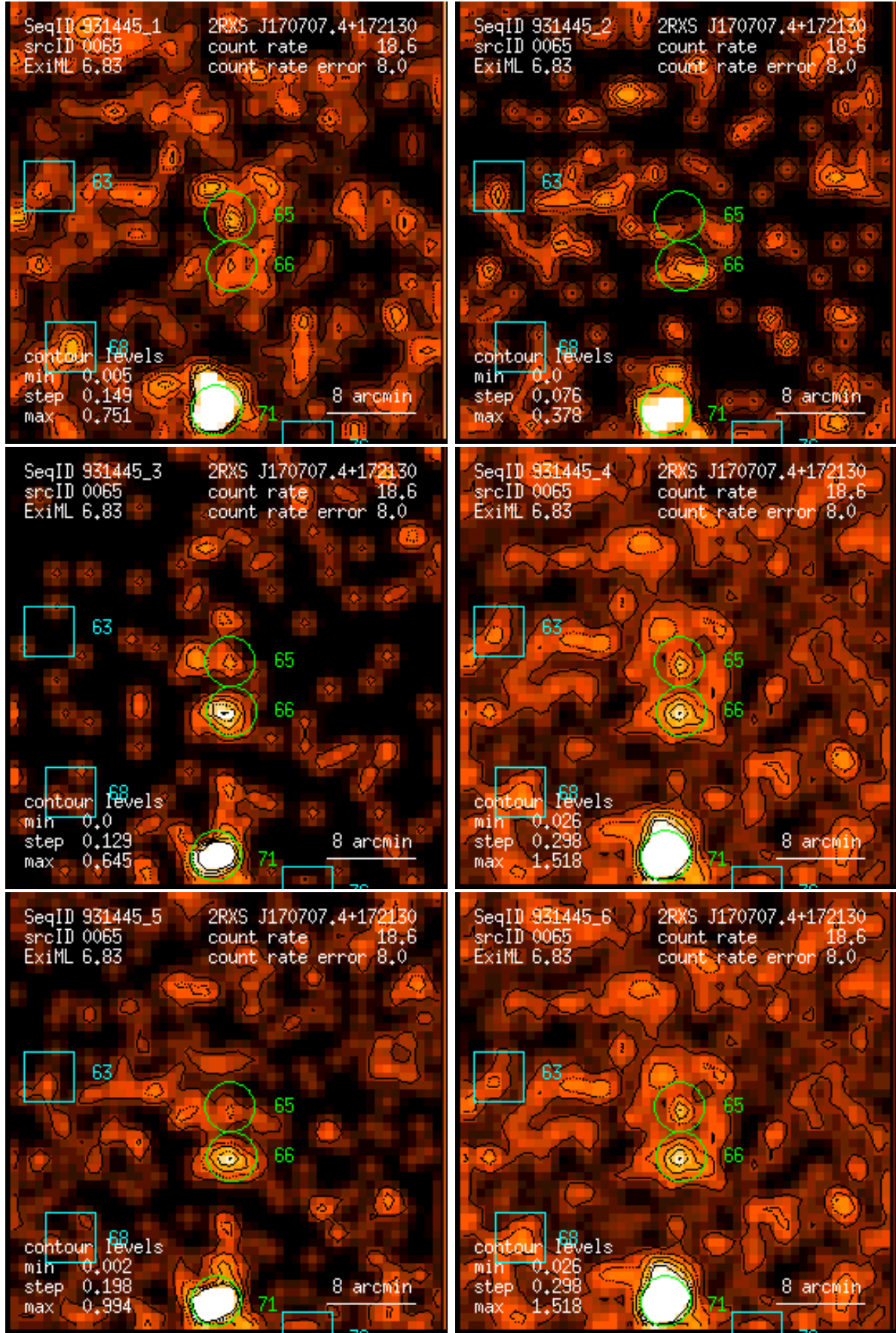
Figure 65: RASS 931445: detection 0065: band rate images, Gaussian filter: (1) PSPC channels 11 – 41, (2) 52 – 90, (3) 91 – 201, (4) 11 – 235, (5) 52 – 201, (6) 11 – 201. Broad band rates in counts/ks. Band rate contour levels in counts/ks/arcmin 2 .
