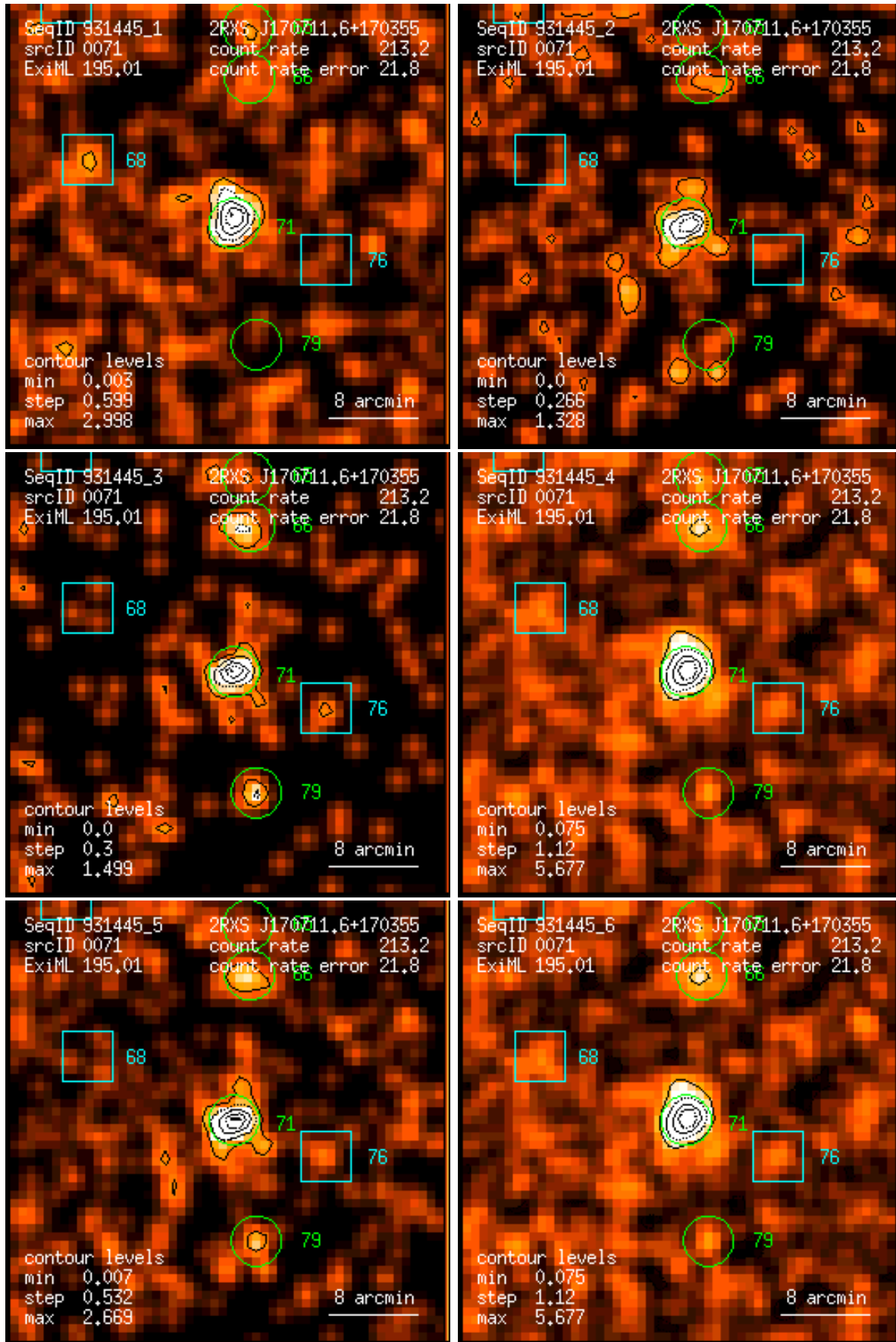
Figure 71: RASS 931445: detection 0071: band rate images, Gaussian filter: (1) PSPC channels 11 – 41, (2) 52 – 90, (3) 91 – 201, (4) 11 – 235, (5) 52 – 201, (6) 11 – 201. Broad band rates in counts/ks. Band rate contour levels in counts/ks/arcmin 2 .
