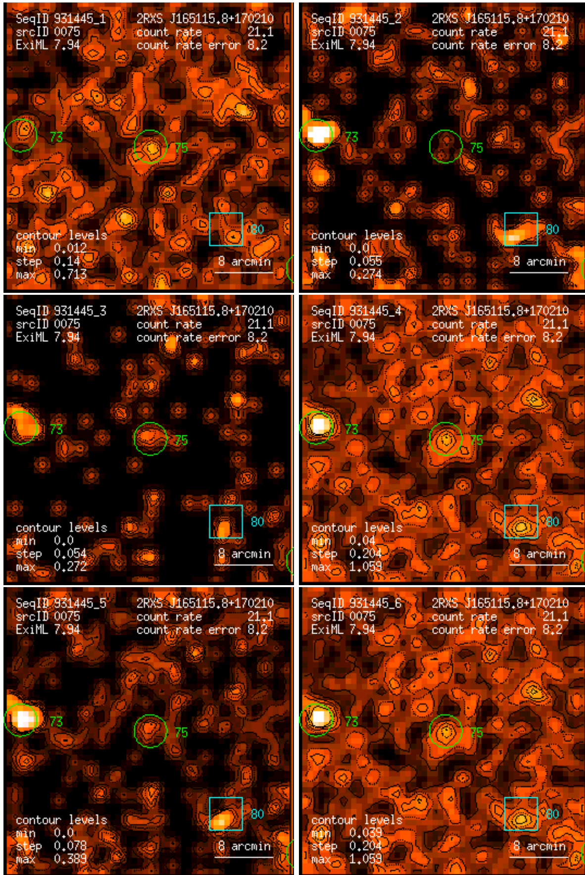
Figure 75: RASS 931445: detection 0075: band rate images, Gaussian filter: (1) PSPC channels 11 – 41, (2) 52 – 90, (3) 91 – 201, (4) 11 – 235, (5) 52 – 201, (6) 11 – 201. Broad band rates in counts/ks. Band rate contour levels in counts/ks/arcmin 2 .
