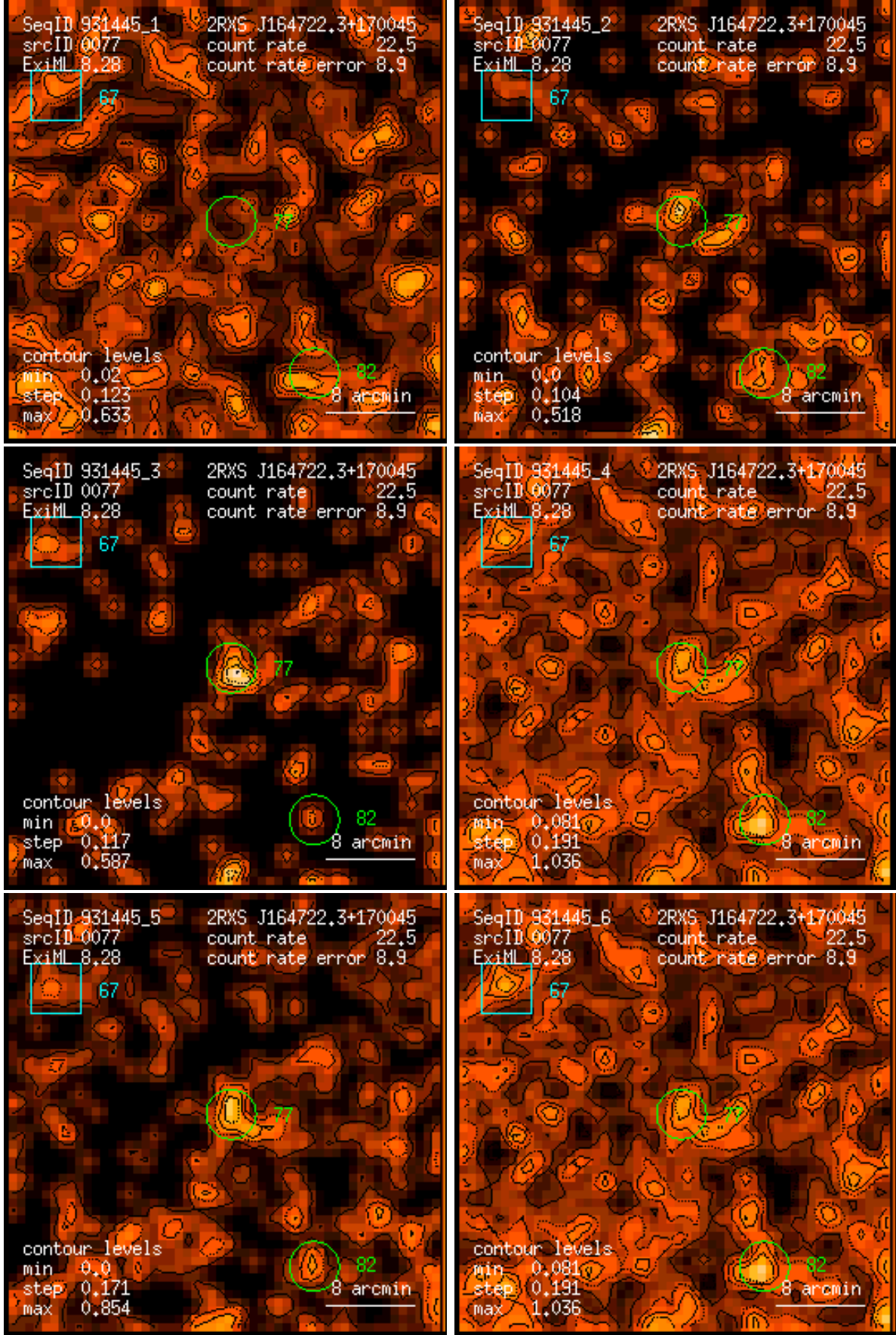
Figure 77: RASS 931445: detection 0077: band rate images, Gaussian filter: (1) PSPC channels 11 – 41, (2) 52 – 90, (3) 91 – 201, (4) 11 – 235, (5) 52 – 201, (6) 11 – 201. Broad band rates in counts/ks. Band rate contour levels in counts/ks/arcmin 2 .
