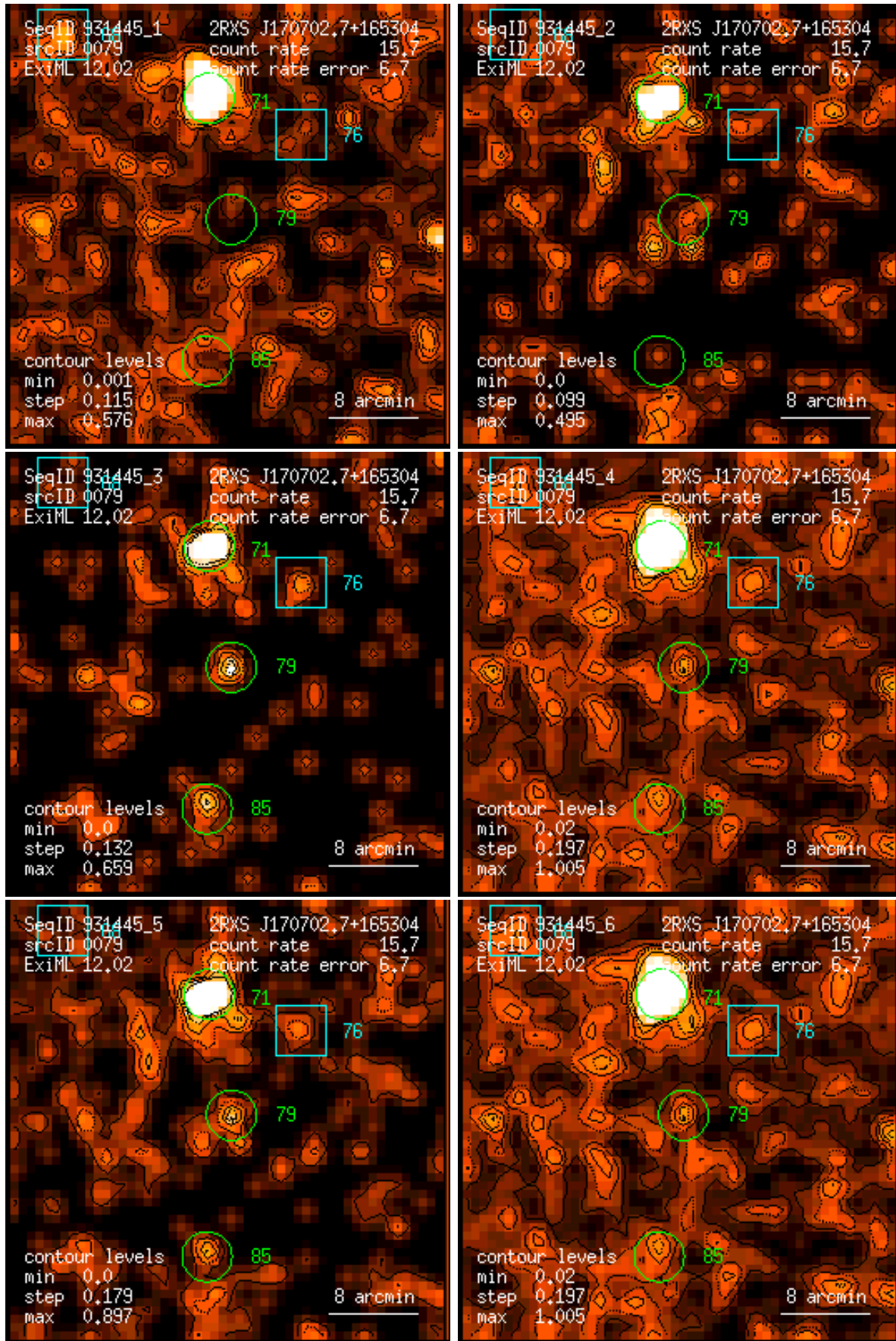
Figure 79: RASS 931445: detection 0079: band rate images, Gaussian filter: (1) PSPC channels 11 – 41, (2) 52 – 90, (3) 91 – 201, (4) 11 – 235, (5) 52 – 201, (6) 11 – 201. Broad band rates in counts/ks. Band rate contour levels in counts/ks/arcmin 2 .
