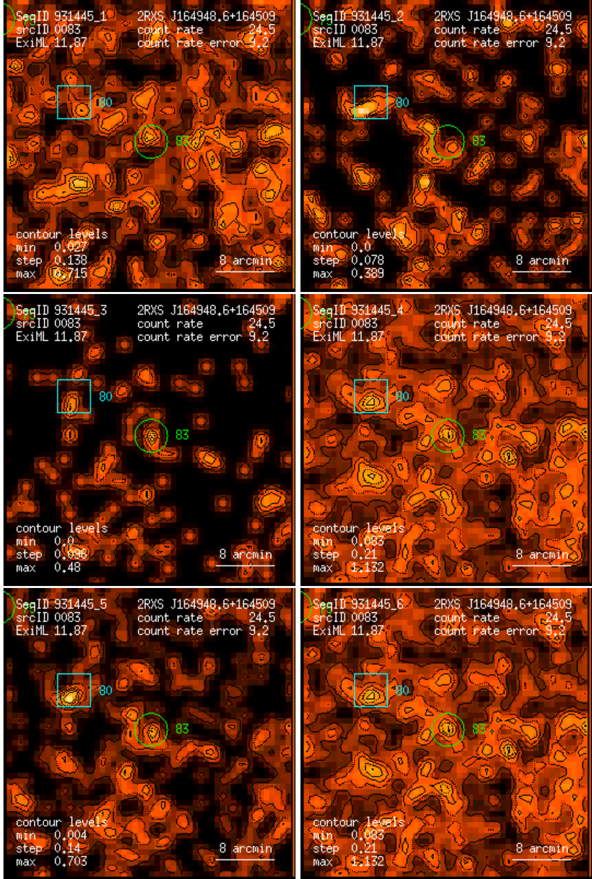
Figure 83: RASS 931445: detection 0083: band rate images, Gaussian filter: (1) PSPC channels 11 – 41, (2) 52 – 90, (3) 91 – 201, (4) 11 – 235, (5) 52 – 201, (6) 11 – 201. Broad band rates in counts/ks. Band rate contour levels in counts/ks/arcmin 2 .
