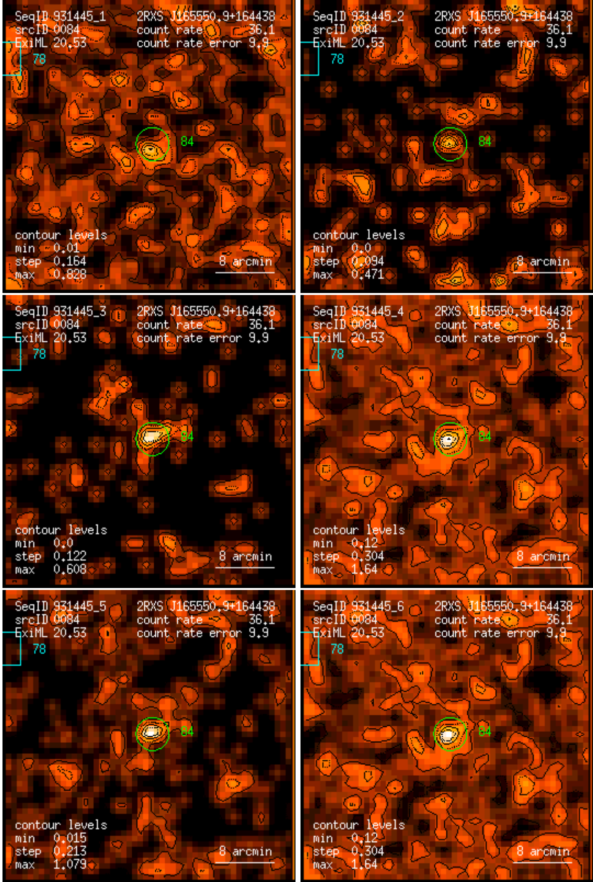
Figure 84: RASS 931445: detection 0084: band rate images, Gaussian filter: (1) PSPC channels 11 – 41, (2) 52 – 90, (3) 91 – 201, (4) 11 – 235, (5) 52 – 201, (6) 11 – 201. Broad band rates in counts/ks. Band rate contour levels in counts/ks/arcmin 2 .
