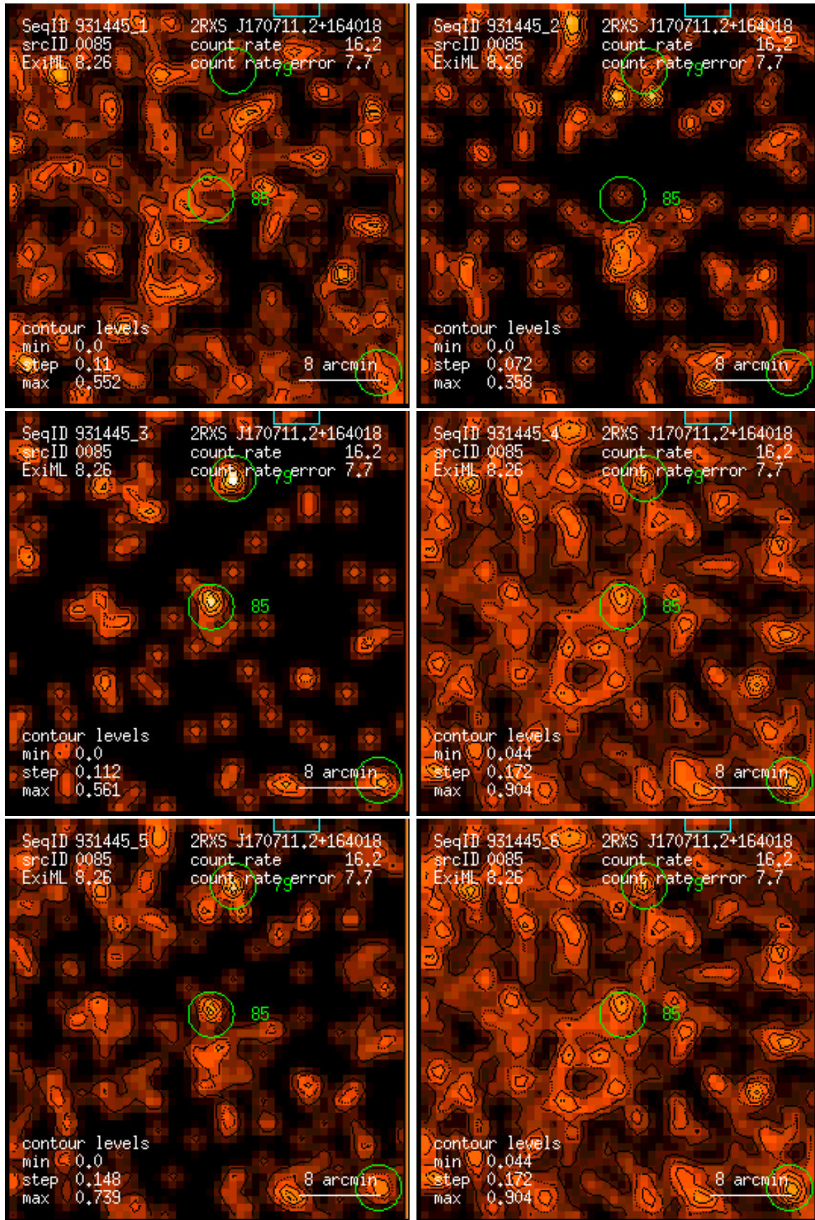
Figure 85: RASS 931445: detection 0085: band rate images, Gaussian filter: (1) PSPC channels 11 – 41, (2) 52 – 90, (3) 91 – 201, (4) 11 – 235, (5) 52 – 201, (6) 11 – 201. Broad band rates in counts/ks. Band rate contour levels in counts/ks/arcmin 2 .
