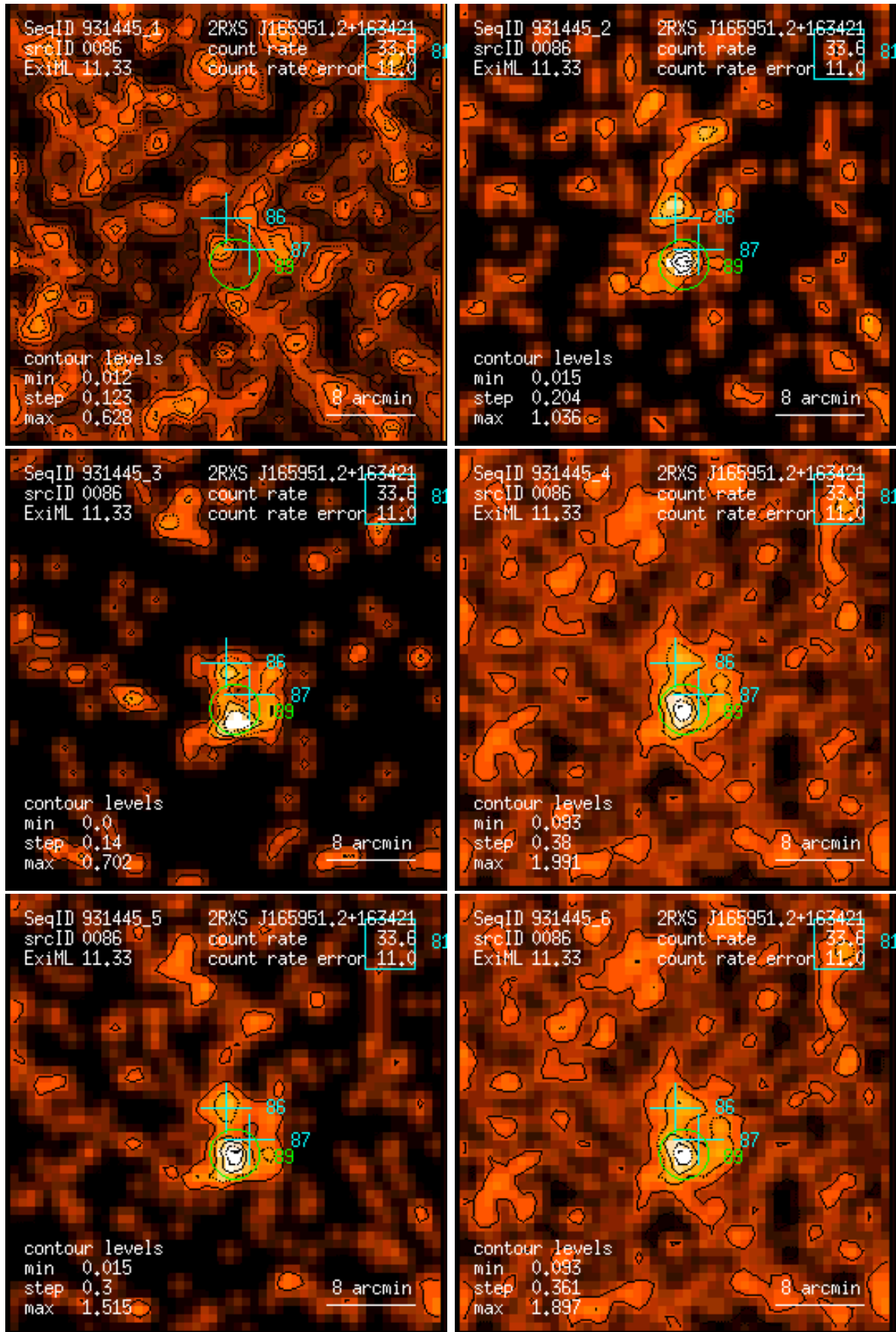
Figure 86: RASS 931445: detection 0086: band rate images, Gaussian filter: (1) PSPC channels 11 – 41, (2) 52 – 90, (3) 91 – 201, (4) 11 – 235, (5) 52 – 201, (6) 11 – 201. Broad band rates in counts/ks. Band rate contour levels in counts/ks/arcmin 2 .
