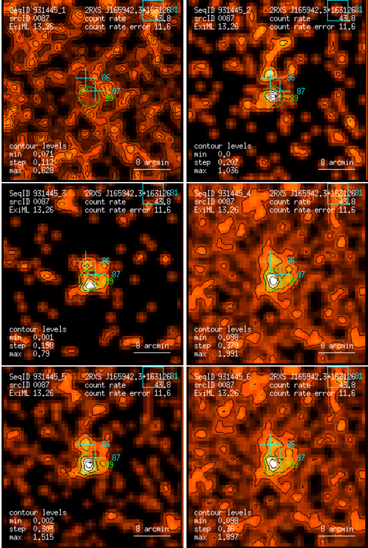
Figure 87: RASS 931445: detection 0087: band rate images, Gaussian filter: (1) PSPC channels 11 – 41, (2) 52 – 90, (3) 91 – 201, (4) 11 – 235, (5) 52 – 201, (6) 11 – 201. Broad band rates in counts/ks. Band rate contour levels in counts/ks/arcmin 2 .
