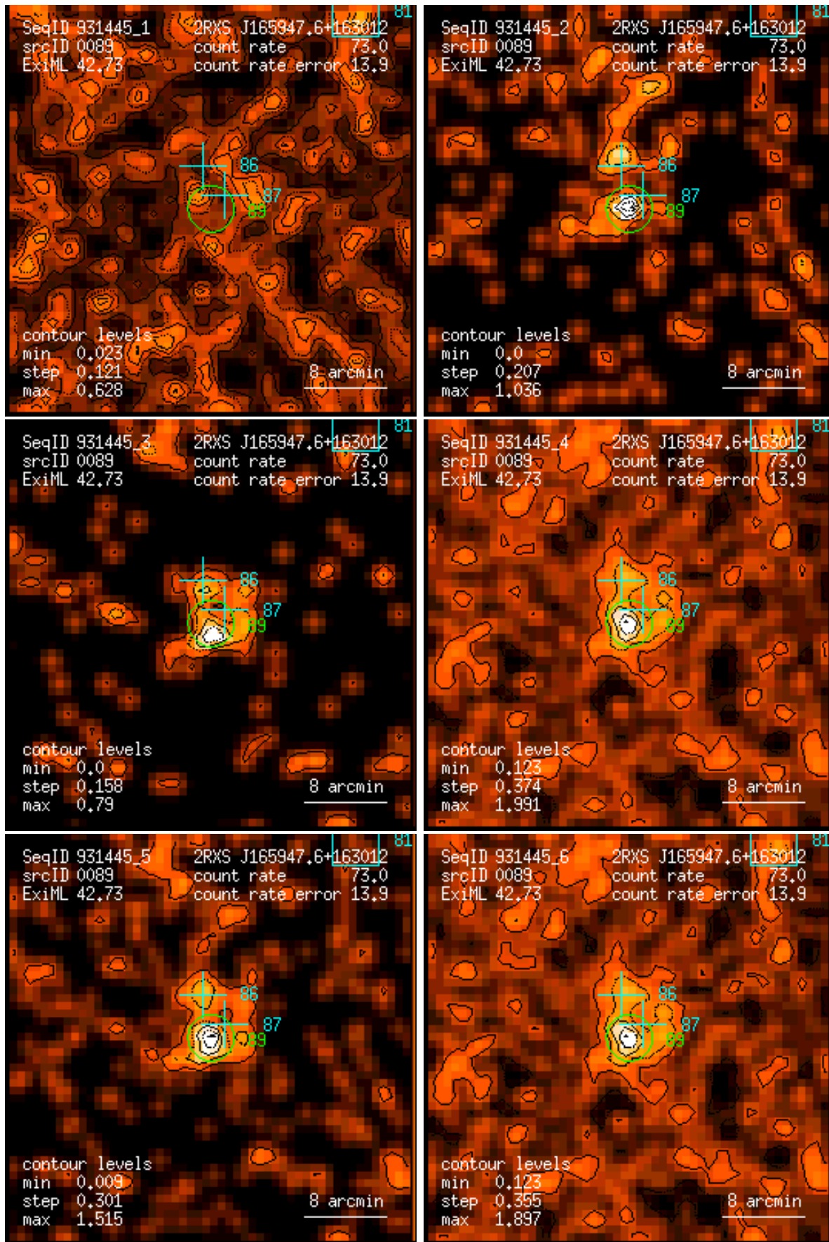
Figure 89: RASS 931445: detection 0089: band rate images, Gaussian filter: (1) PSPC channels 11 – 41, (2) 52 – 90, (3) 91 – 201, (4) 11 – 235, (5) 52 – 201, (6) 11 – 201. Broad band rates in counts/ks. Band rate contour levels in counts/ks/arcmin 2 .
