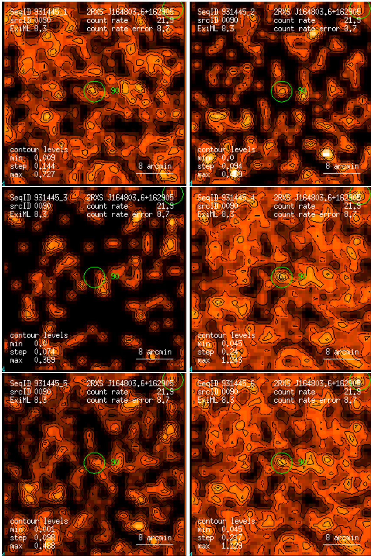
Figure 90: RASS 931445: detection 0090: band rate images, Gaussian filter: (1) PSPC channels 11 – 41, (2) 52 – 90, (3) 91 – 201, (4) 11 – 235, (5) 52 – 201, (6) 11 – 201. Broad band rates in counts/ks. Band rate contour levels in counts/ks/arcmin 2 .
