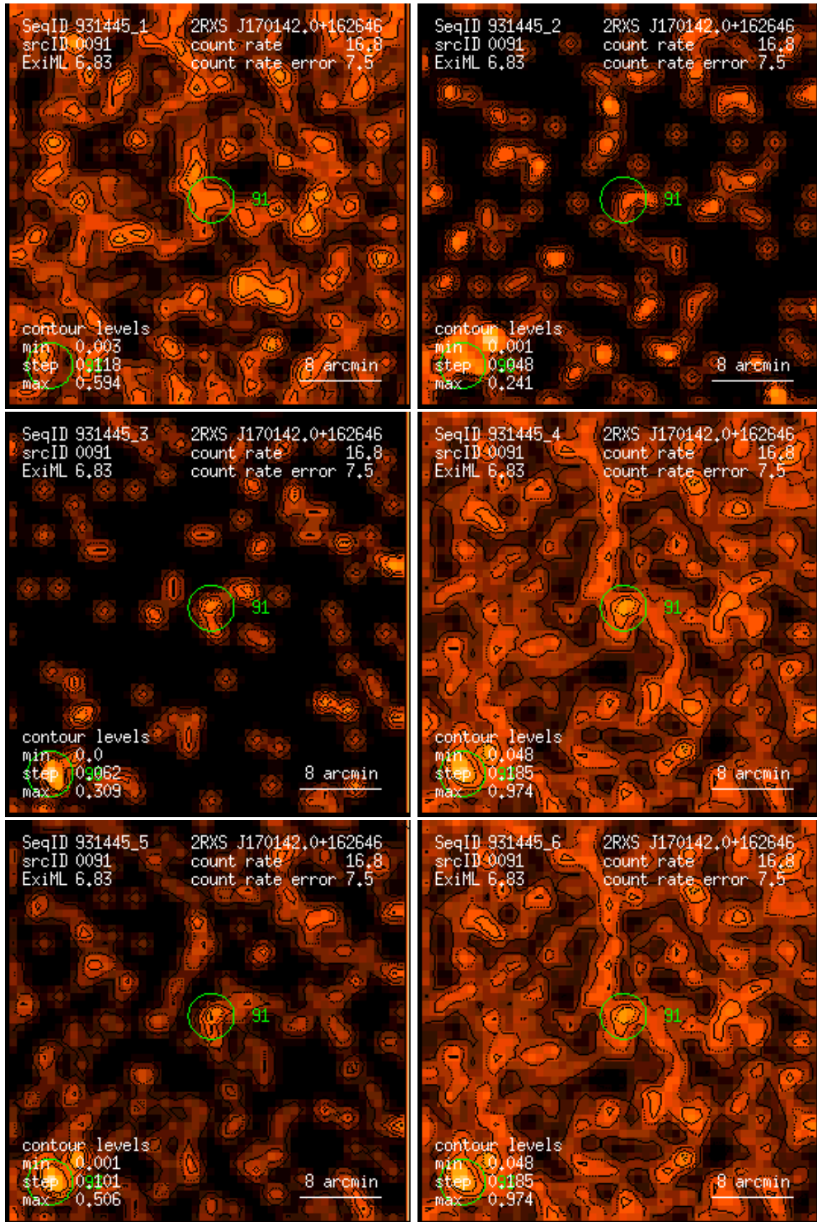
Figure 91: RASS 931445: detection 0091: band rate images, Gaussian filter: (1) PSPC channels 11 – 41, (2) 52 – 90, (3) 91 – 201, (4) 11 – 235, (5) 52 – 201, (6) 11 – 201. Broad band rates in counts/ks. Band rate contour levels in counts/ks/arcmin 2 .
