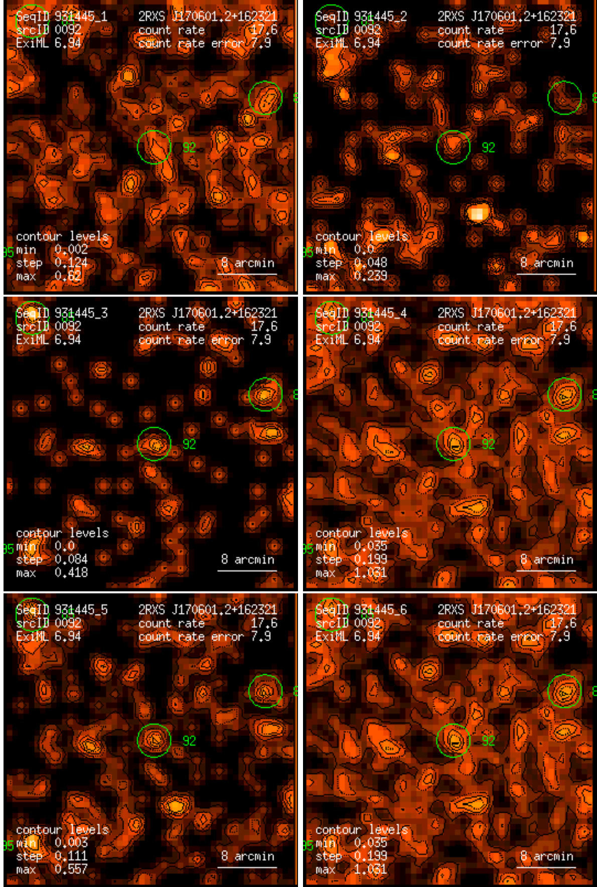
Figure 92: RASS 931445: detection 0092: band rate images, Gaussian filter: (1) PSPC channels 11 – 41, (2) 52 – 90, (3) 91 – 201, (4) 11 – 235, (5) 52 – 201, (6) 11 – 201. Broad band rates in counts/ks. Band rate contour levels in counts/ks/arcmin 2 .
