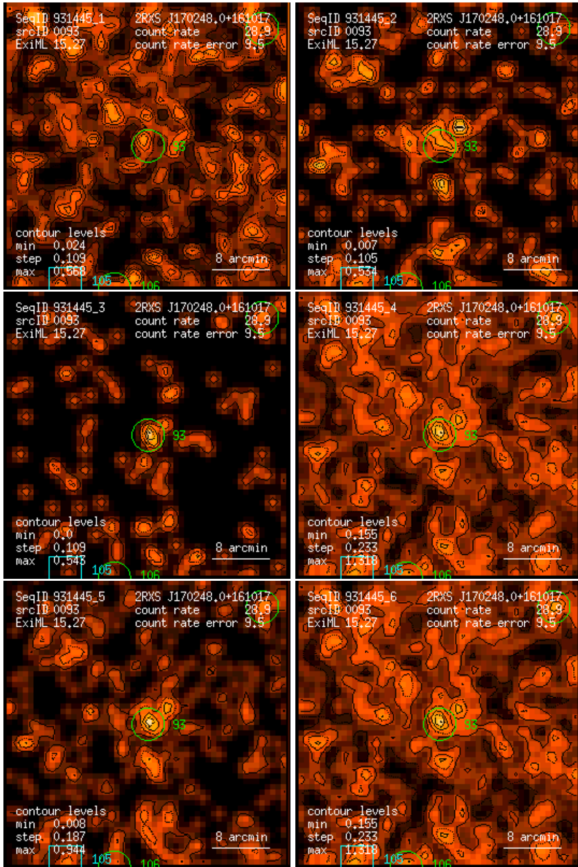
Figure 93: RASS 931445: detection 0093: band rate images, Gaussian filter: (1) PSPC channels 11 – 41, (2) 52 – 90, (3) 91 – 201, (4) 11 – 235, (5) 52 – 201, (6) 11 – 201. Broad band rates in counts/ks. Band rate contour levels in counts/ks/arcmin 2 .
