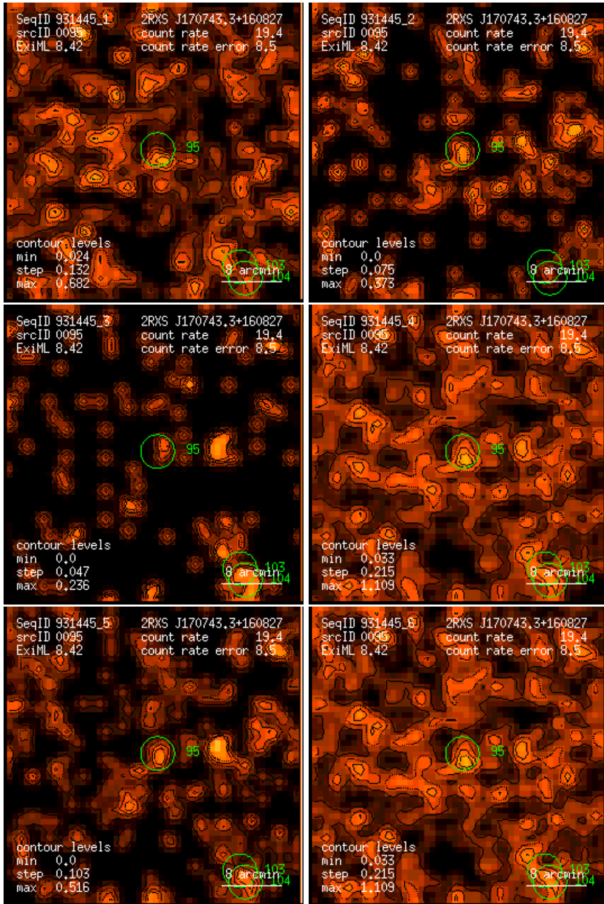
Figure 95: RASS 931445: detection 0095: band rate images, Gaussian filter: (1) PSPC channels 11 – 41, (2) 52 – 90, (3) 91 – 201, (4) 11 – 235, (5) 52 – 201, (6) 11 – 201. Broad band rates in counts/ks. Band rate contour levels in counts/ks/arcmin 2 .
