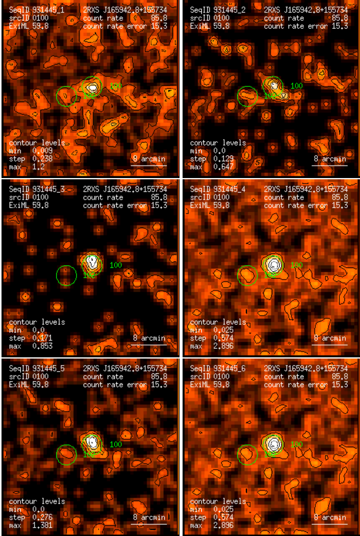
Figure 100: RASS 931445: detection 0100: band rate images, Gaussian filter: (1) PSPC channels 11 – 41, (2) 52 – 90, (3) 91 – 201, (4) 11 – 235, (5) 52 – 201, (6) 11 – 201. Broad band rates in counts/ks. Band rate contour levels in counts/ks/arcmin 2 .
