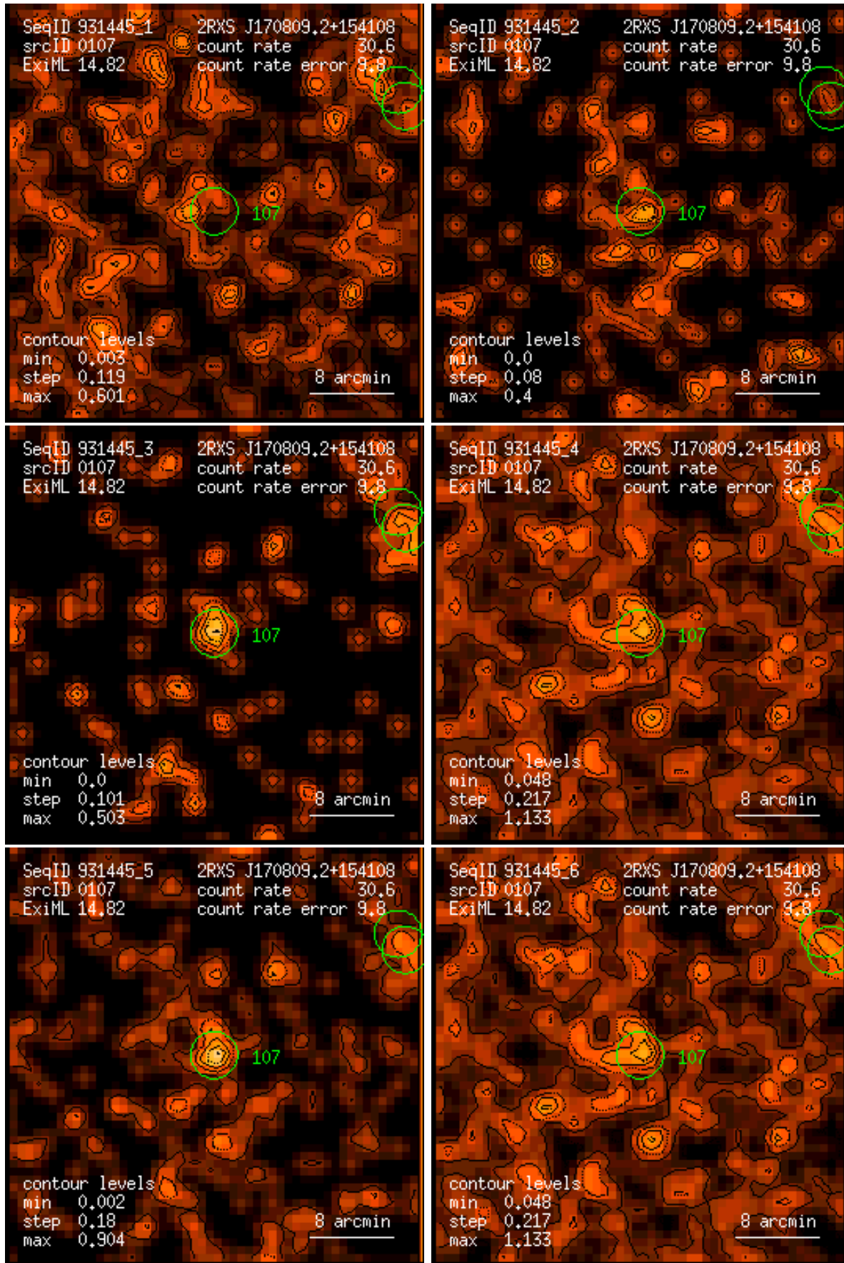
Figure 107: RASS 931445: detection 0107: band rate images, Gaussian filter: (1) PSPC channels 11 – 41, (2) 52 – 90, (3) 91 – 201, (4) 11 – 235, (5) 52 – 201, (6) 11 – 201. Broad band rates in counts/ks. Band rate contour levels in counts/ks/arcmin 2 .
