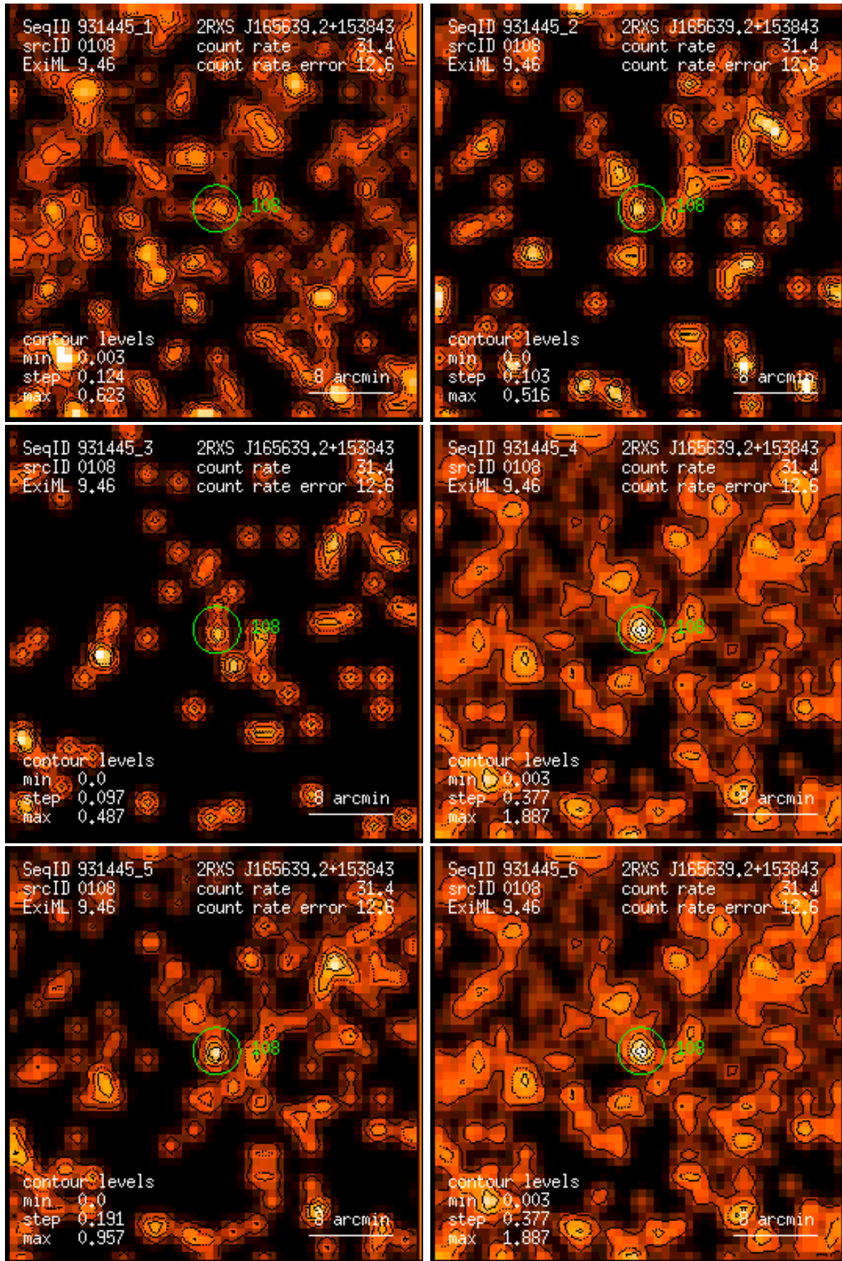
Figure 108: RASS 931445: detection 0108: band rate images, Gaussian filter: (1) PSPC channels 11 – 41, (2) 52 – 90, (3) 91 – 201, (4) 11 – 235, (5) 52 – 201, (6) 11 – 201. Broad band rates in counts/ks. Band rate contour levels in counts/ks/arcmin 2 .
