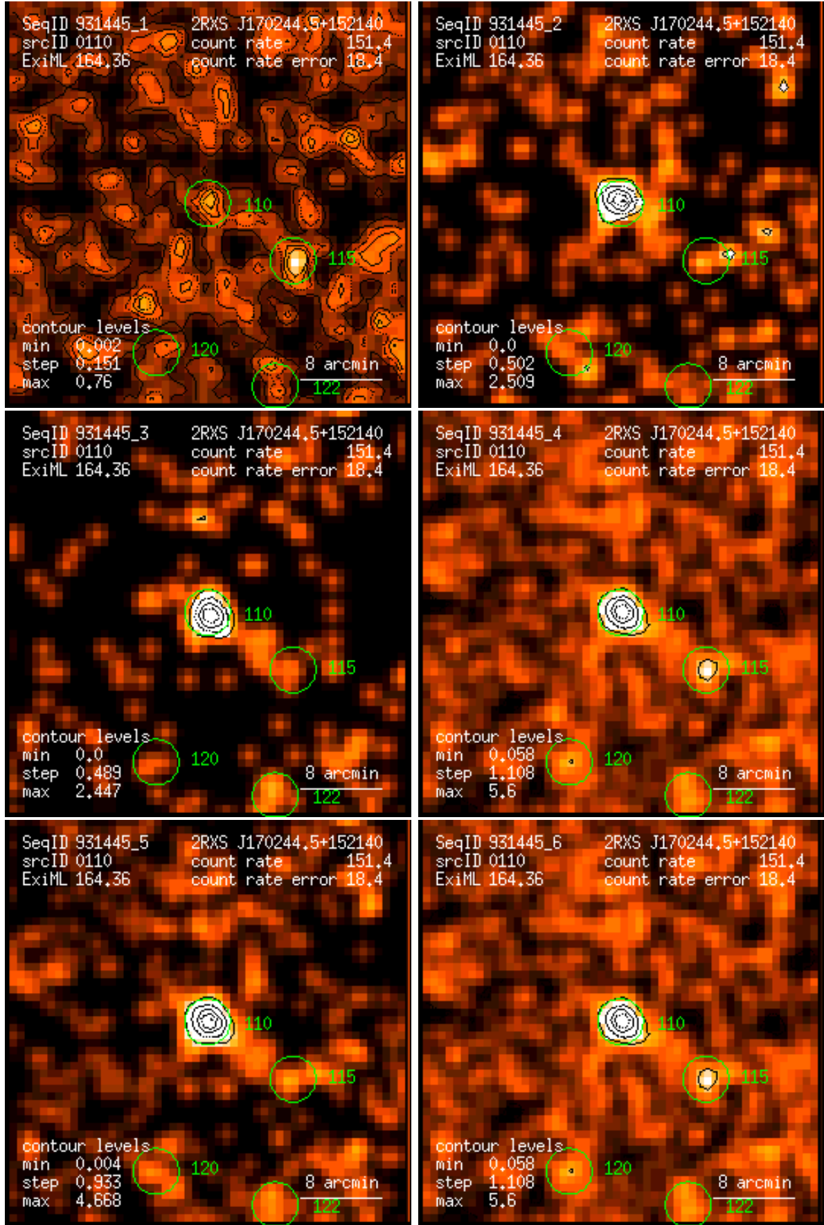
Figure 110: RASS 931445: detection 0110: band rate images, Gaussian filter: (1) PSPC channels 11 – 41, (2) 52 – 90, (3) 91 – 201, (4) 11 – 235, (5) 52 – 201, (6) 11 – 201. Broad band rates in counts/ks. Band rate contour levels in counts/ks/arcmin 2 .
