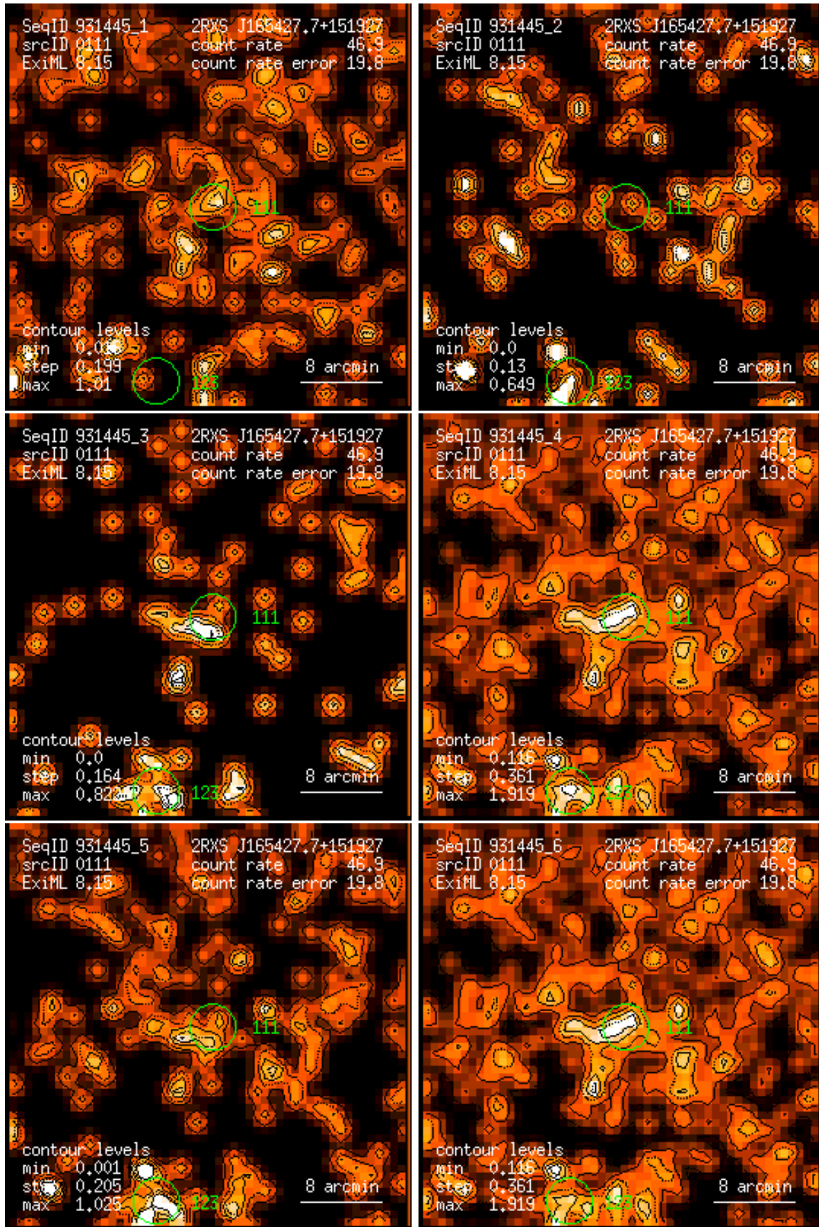
Figure 111: RASS 931445: detection 0111: band rate images, Gaussian filter: (1) PSPC channels 11 – 41, (2) 52 – 90, (3) 91 – 201, (4) 11 – 235, (5) 52 – 201, (6) 11 – 201. Broad band rates in counts/ks. Band rate contour levels in counts/ks/arcmin 2 .
